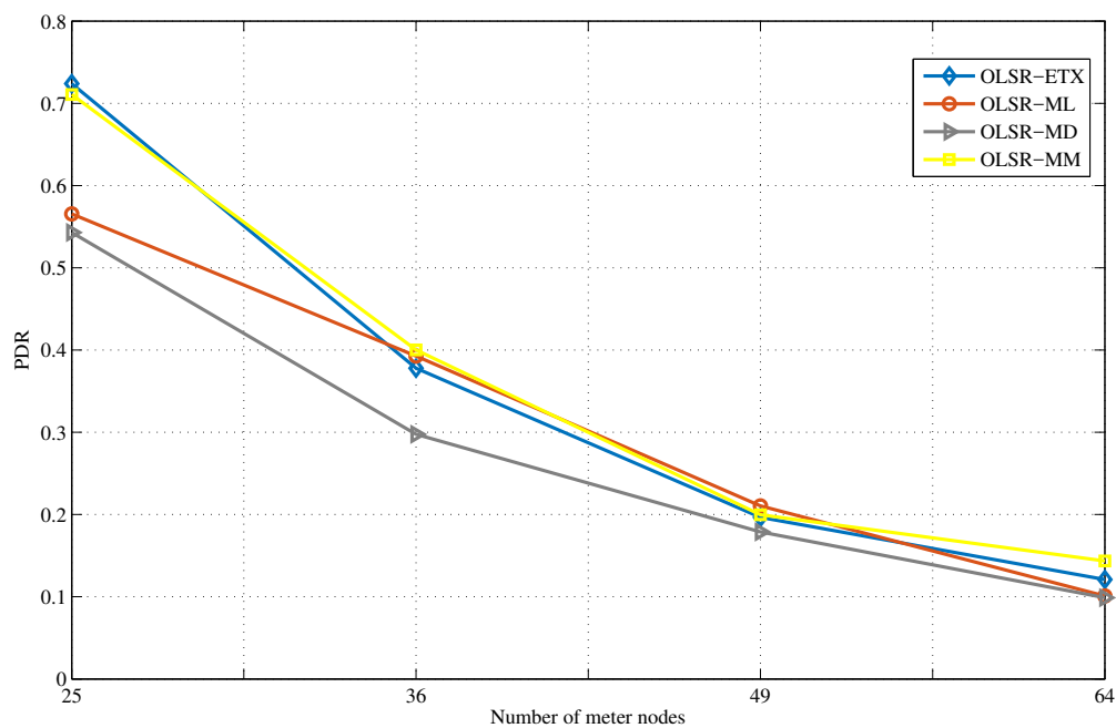
Figure 12. PDR for smart grid application on grid clusters with a central placement of the data concentrator.
