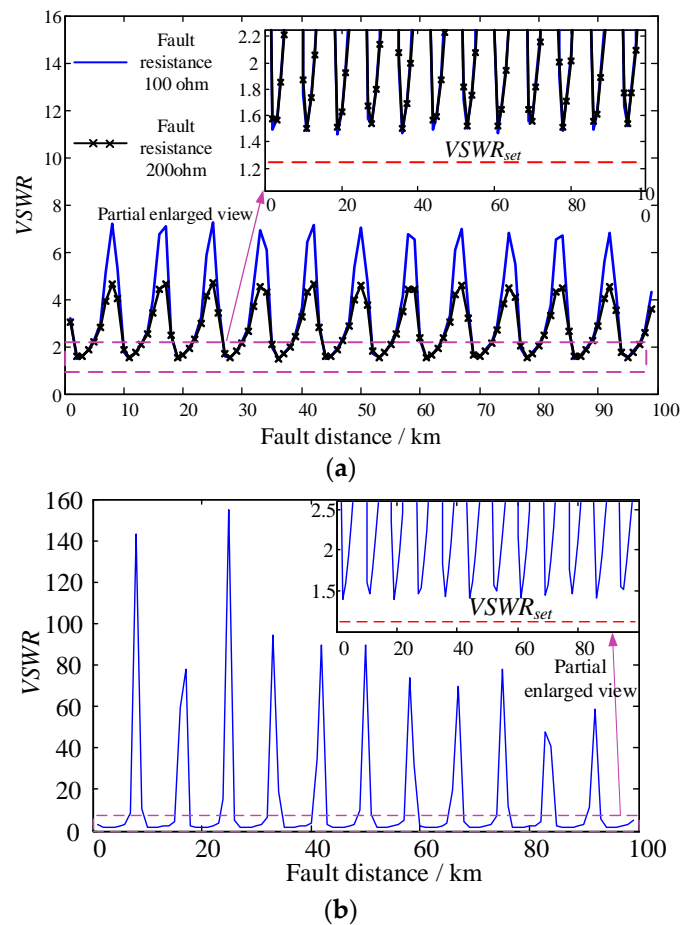
Figure 10. The VSWR for different fault position of single-line earth fault with matched terminal resistor. (a) the transition resistance are 100 Ω and 200 Ω, respectively; (b) the transition resistance is 0.1 Ω.
