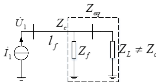
Figure 8. Non-metallic short circuit with mismatching terminal resistor.
