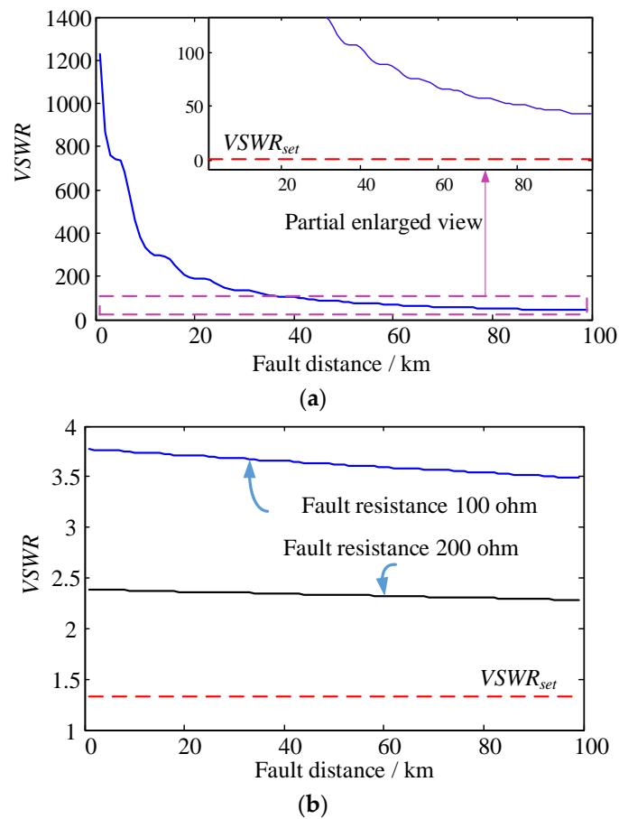
Figure 9. The VSWR for different fault position of double-line earth fault with matched terminal resistor. (a) the transition resistance is 0.1 Ω; (b) the transition resistance are 100 Ω and 200 Ω, respectively.
