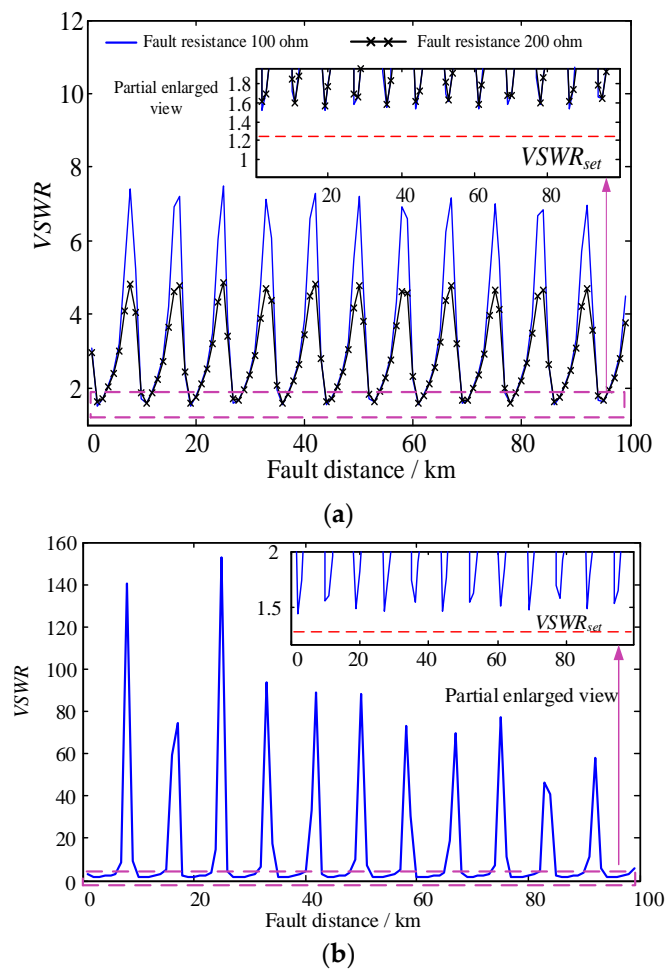
Figure 12. The VSWR for different fault position of single-line earth fault with mismatched terminal resistor. (a) the transition resistance are 100 \Omega and 200 \Omega , respectively; (b) the transition resistance is 0.1 \Omega .
