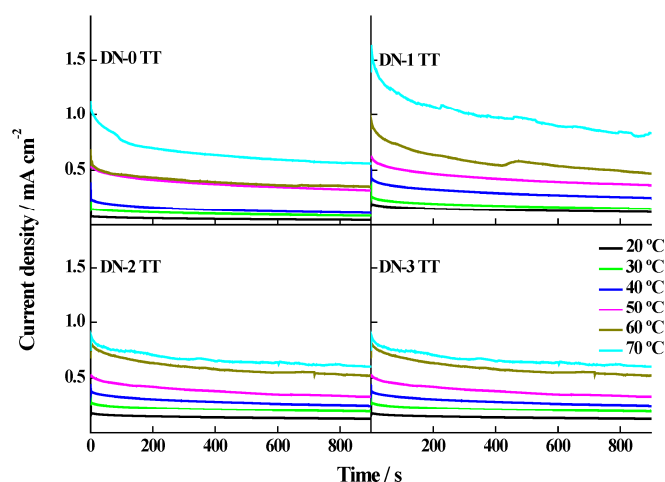
Figure 9. i-t curves for the methanol oxidation on the synthesized Pt-Ru catalysts. Scan rate: 20 mV·s -1 . Supporting electrolyte: 0.5 M H 2 SO 4 . Methanol concentration: 2.0 M. Applied potential: 0.55 V vs. RHE.
