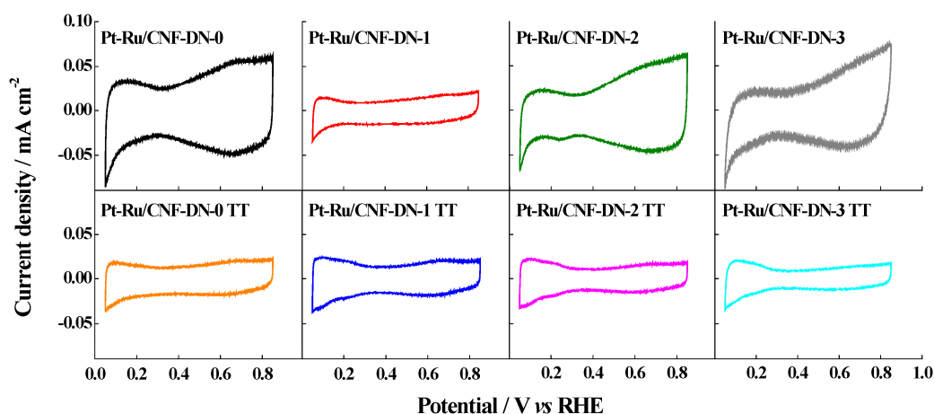
Figure 6. CVs in 0.5 M H 2 SO 4 (supporting electrolyte) recorded at 20 mV·s -1 .
