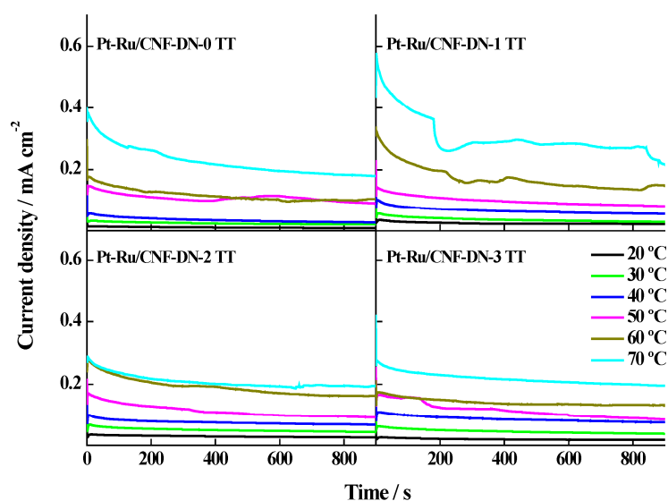
Figure 8. i-t curves for methanol oxidation on the synthesized Pt-Ru catalysts. Scan rate: 20 \text{ mV}\cdot\text{s}^{-1} . Supporting electrolyte: 0.5 \text{ M H}_2\text{SO}_4 . Methanol concentration: 2.0 \text{ M} . Applied potential: 0.45 \text{ V} vs. RHE.
