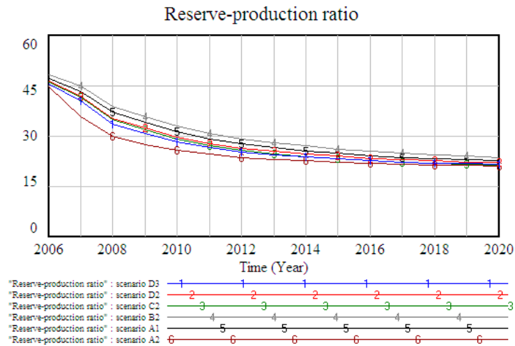
Figure 13. Reserve/production ratio.
