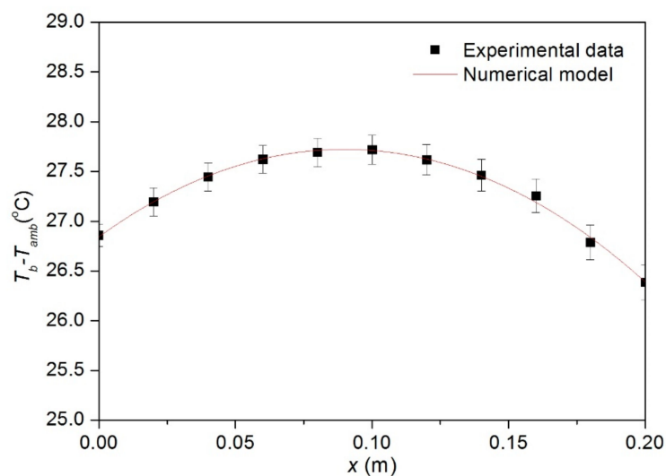
Figure A1. Comparison of temperature differences from experimental data and results of the numerical model for L_h/L of 1, channel width of 3 mm, flow rate of 0 \text{ m}^3/\text{min} , and heat input of 5 W.
