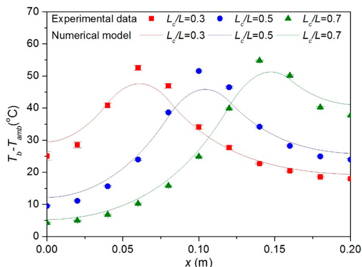
Figure A2. Comparison of temperature differences from experimental data and results of the numerical model for L_h/L of 0.2, channel width of 7 mm, and flow rate of 0.2 \text{ m}^3/\text{min} .
