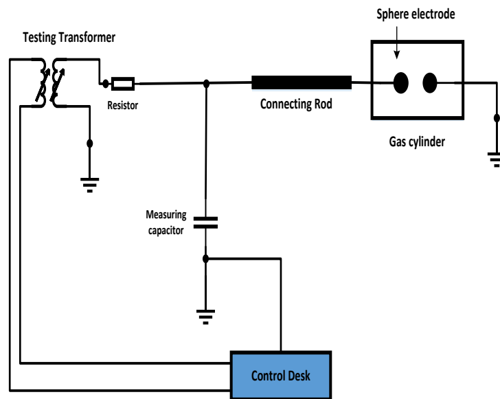
Figure 1. Schematic to examine R152a/CO 2 breakdown voltage by sphere–sphere electrodes.
