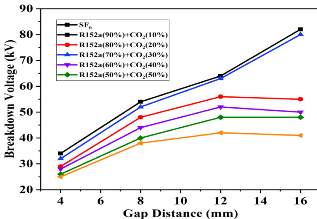
Figure 5. Breakdown voltages of R152a/CO 2 gas varying the gap distance (4–16 mm) at different mixture ratio.
