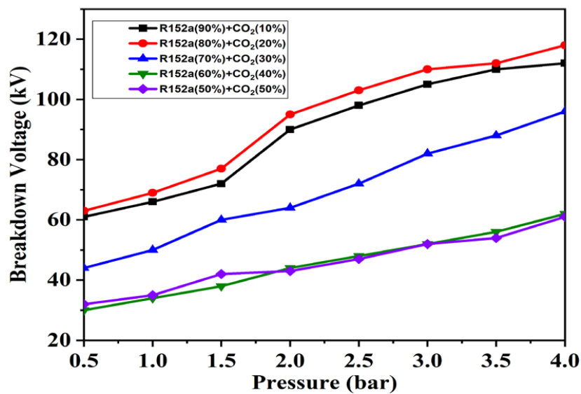
Figure 6. DC breakdown voltage characteristics of R152a/CO 2 with different mixture ratios and 8 mm gap distance.
