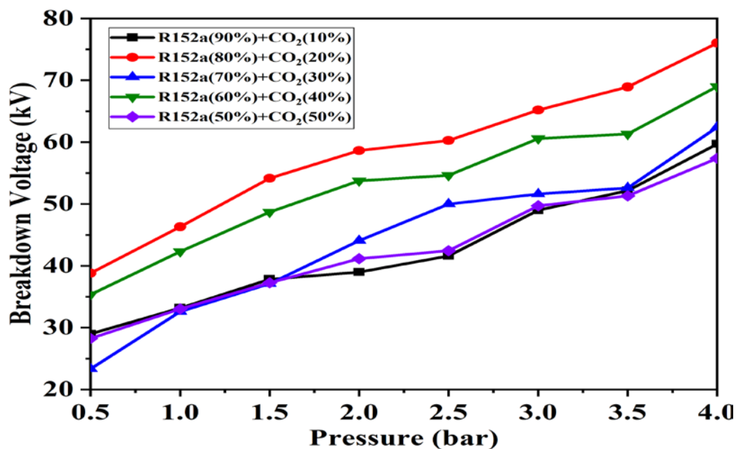
Figure 3. AC power frequency breakdown voltage of R152a/CO 2 gas at varying mixture ratio and 8 mm electrode gap distance.
