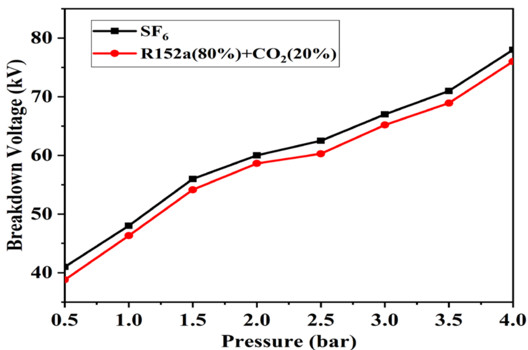
Figure 4. Breakdown characteristic comparison of R152a/CO 2 gas at 80%/20% mixture ratio and SF 6 at 8 mm electrode gap distance.
