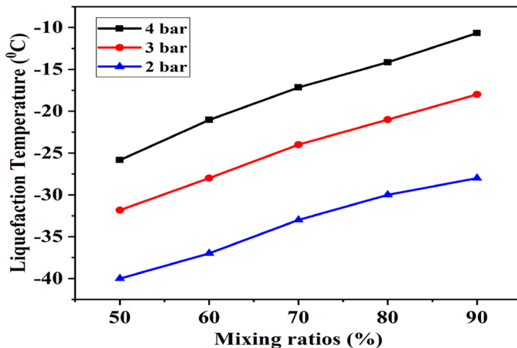
Figure 9. Liquefaction temperature of R152a at different pressure and mixture ratio.
