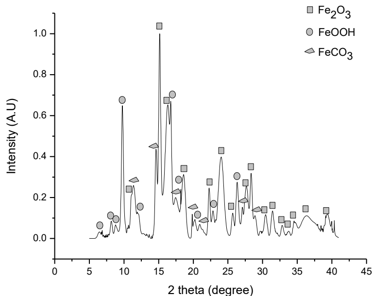
Figure 1. XRD pattern of iron ore sample.
