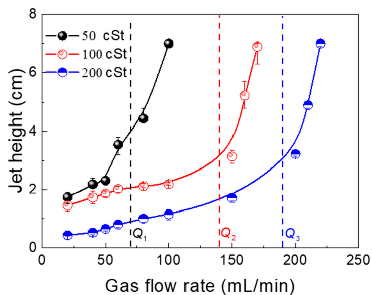
Figure 10. Jet height with different gas flow rates.
