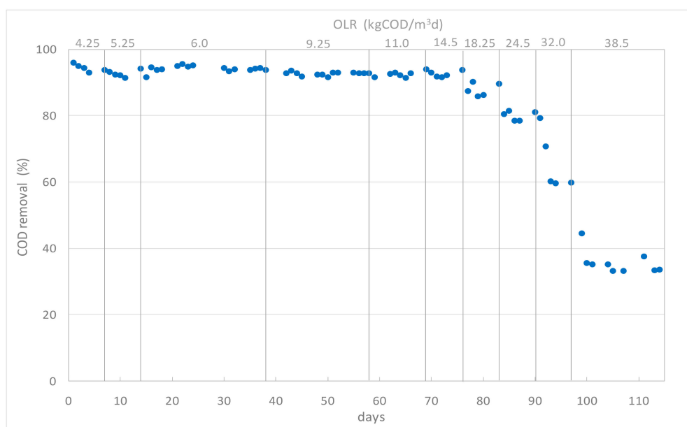
Figure 2. Chemical oxygen demand (COD) removal over the pilot plant operational phase.
