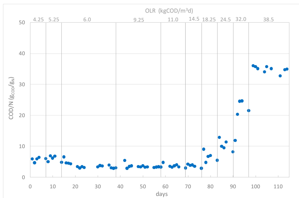
Figure 6. COD/N ratio over the pilot plant operational phase.
