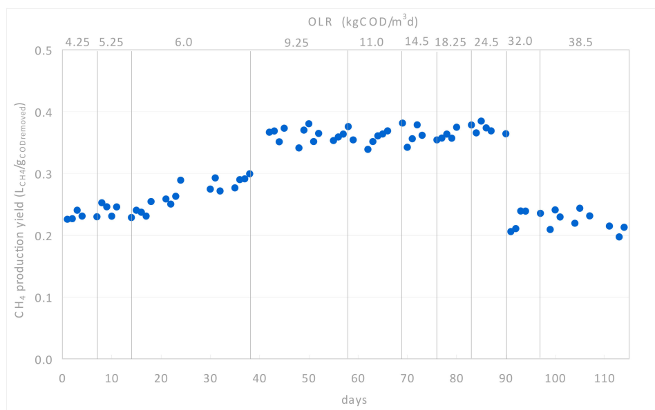
Figure 4. Methane production yield over the pilot plant operational phase.
