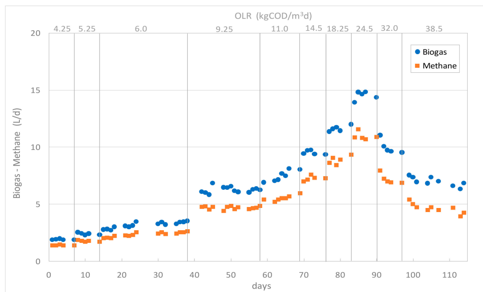
Figure 3. Biogas and methane productions over the pilot plant operational phase.
