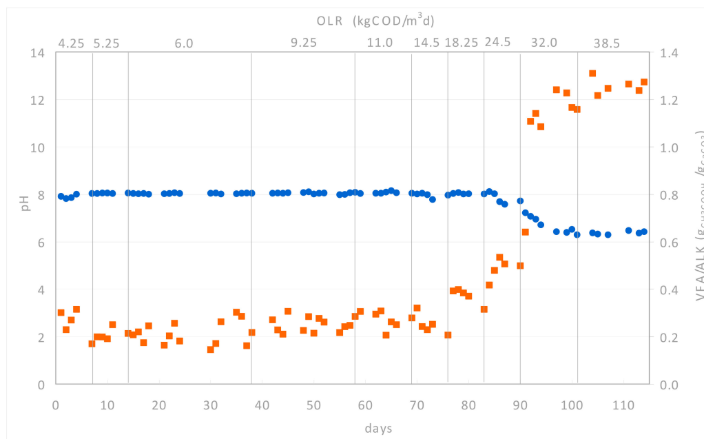
Figure 5. pH and VFA/ALK over the pilot plant operational phase.
