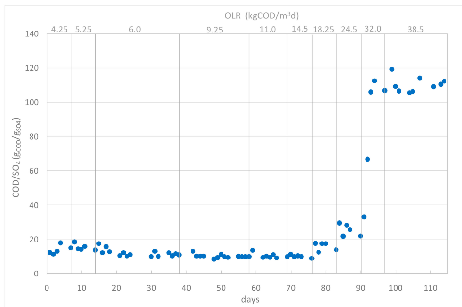
Figure 7. COD/SO 4 ratio over the operational phase of pilot plant.
