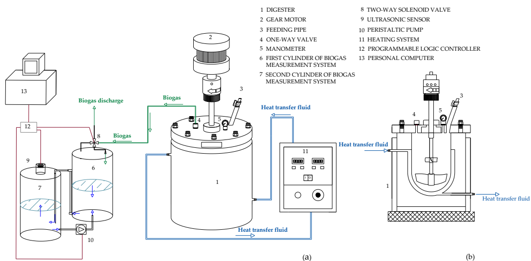
Figure 1. Schematic diagram of pilot plant (a), vertical section of completely stirred tank reactor (CSTR) (b).
