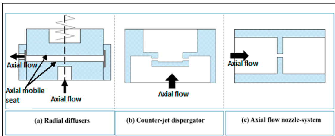
Figure 1. High-pressure homogenization (HPH) disruption units in (a) radial-diffusers; (b) counter-jet-dispergator: jet-dispergator; and (c) axial flow nozzle-system. Reproduced with permission from Gall et al. Processes ; published by MDPI, 2016 [28].
