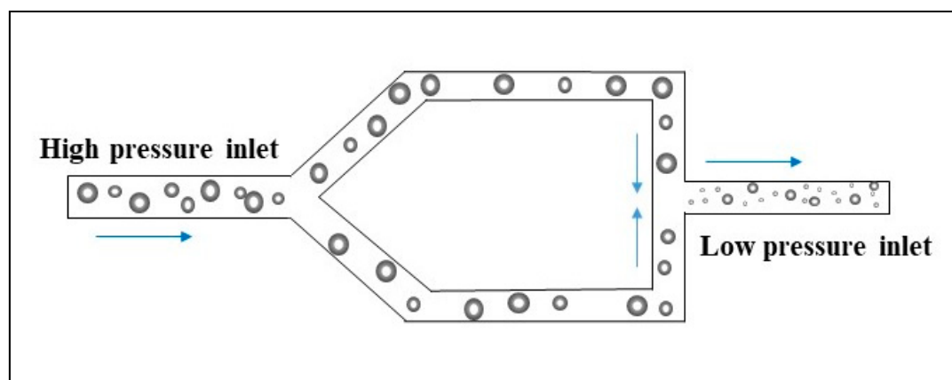
Figure 3. Schematic image of a high pressure microfluidizer.
