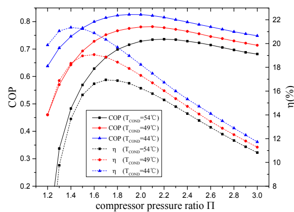
Figure 20. COP and \eta of configuration 1 versus \pi at different T_{COND} .
