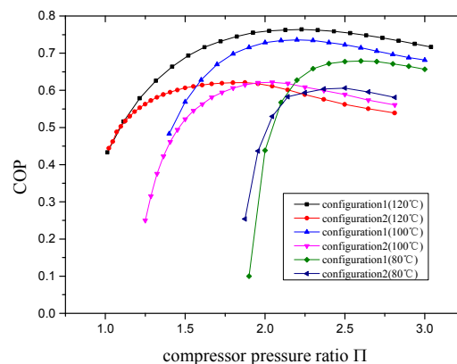
Figure 12. COP versus \pi at different T_{GEN} for both hybrid cycles.
