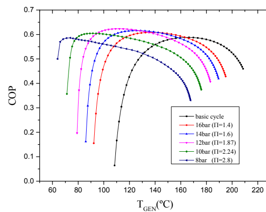
Figure 11. COP versus T_{GEN} for configuration 2 at different intermediate pressures.
