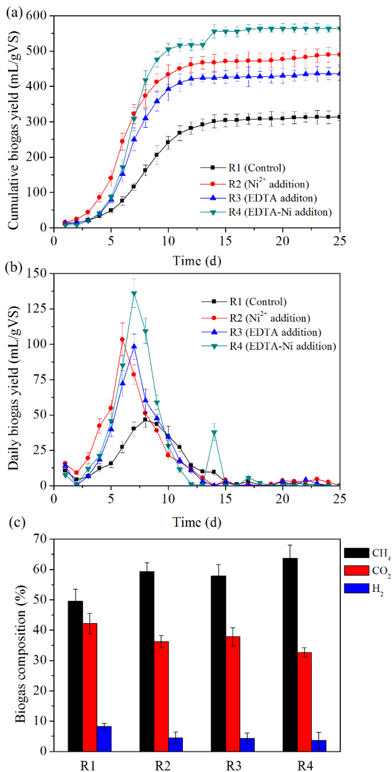
Figure 1. Effect of ethylenediaminetetraacetic acid (EDTA) and/or Ni on (a) cumulative biogas production and (b) daily biogas yield, and (c) biogas composition in the AD of KWs.
