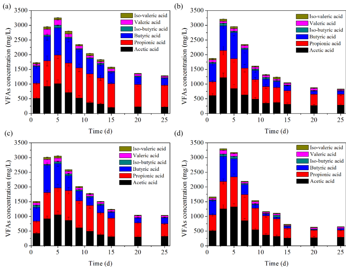
Figure 2. Changes of volatile fatty acids (VFAs) components in (a) R1 (Control test), (b) R2 (with Ni 2+ addition), (c) R3 (with EDTA addition), (d) R4 (with EDTA-Ni addition).
