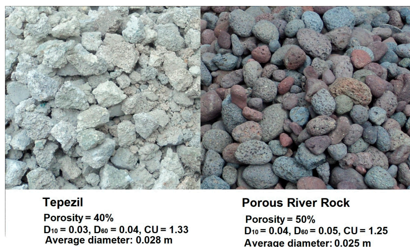
Figure 2. Materials used as filter media in the constructed wetlands (CWs) in this study.
