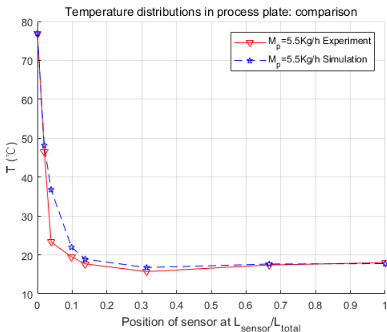
Figure 13. Comparison of inner temperature distribution of Experiment 8 with \dot{M}_p = 152 \text{ kg}\cdot\text{h}^{-1} and T_{u-in} = 15.6 \text{ }^\circ\text{C} .
