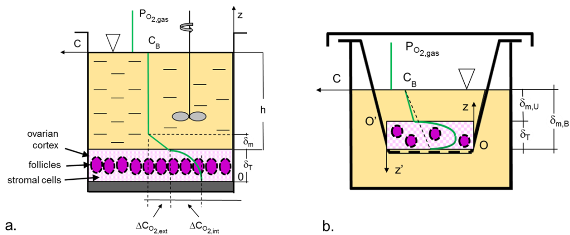
Figure 2. Bioreactor schemes used for the transport models and qualitative dissolved oxygen concentration profile in the medium and inside the fragment: (a) conventional or mixed dish in which oxygen is supplied only through the upper fragment surface, and (b) submerged fragment culture on a permeable membrane at the bottom of an insert suspended in a well of a 24-well plate. Captions: C —dissolved oxygen concentration; C_B —dissolved oxygen concentration in the medium at equilibrium with pO_{2,gas} ; pO_{2,gas} —gaseous oxygen tension above the medium surface; \delta_m and \delta_{m,U} or \delta_{m,B} —thickness of the medium layer above or below the strip, respectively; \delta_T —thickness of the tissue fragment; \Delta CO_{2,ext} —external dissolved oxygen concentration drop in the medium; \Delta CO_{2,int} —internal dissolved oxygen concentration drop in the fragment. Other symbols are defined in the text. Please note that drawings are not to scale.
