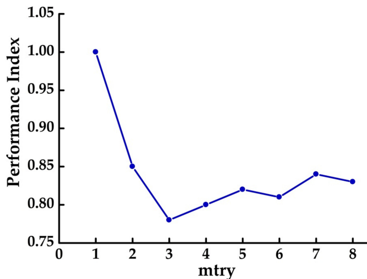
Figure 5. Results for RF trained with different number of randomly selected variables to grow the tree ( mtry ) selections.
