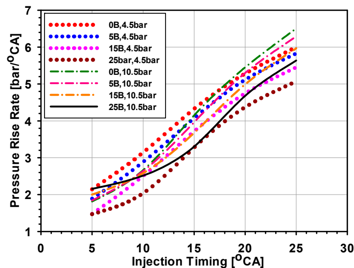
Figure 4. Variation of pressure rise rate with injection timing for diesel and butanol blends at BMEP = 4.5 bar and 10.5 bar.
