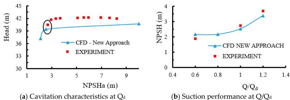
Figure 11. Suction performance prediction and comparison.
