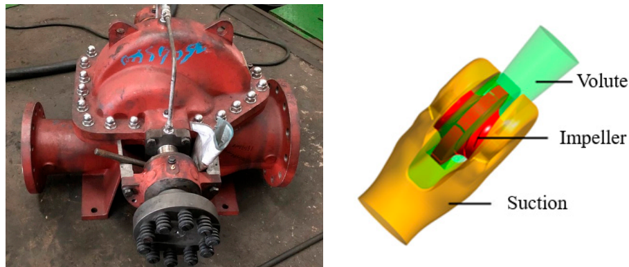
Figure 1. Tested pump and computational domain.
