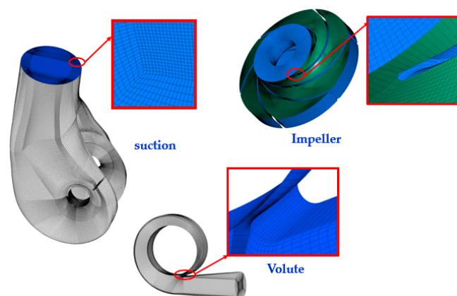
Figure 2. Mesh overview of the flow domains.
