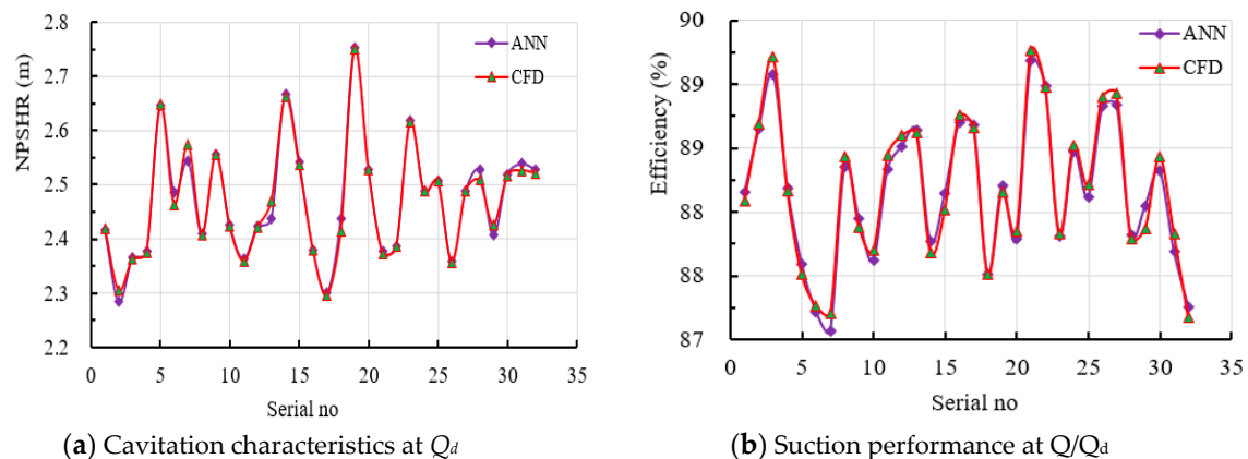
Figure 14. Validation of ANN prediction with CFD.
