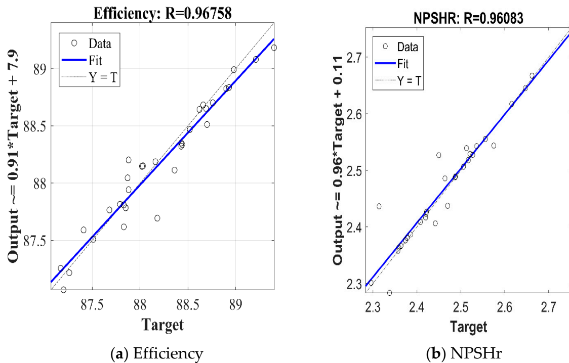
Figure 13. R-Square analysis of efficiency and NPSHr.
