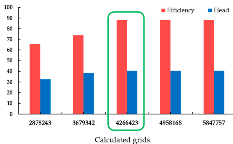
Figure 3. Performance comparison for 5 independent grids.
