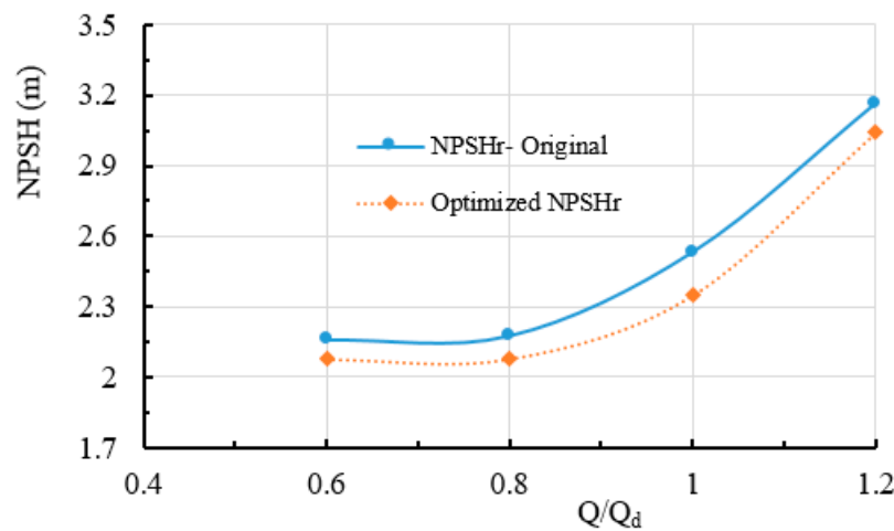
Figure 16. Predicted NPSHr comparison at different flow rates.
