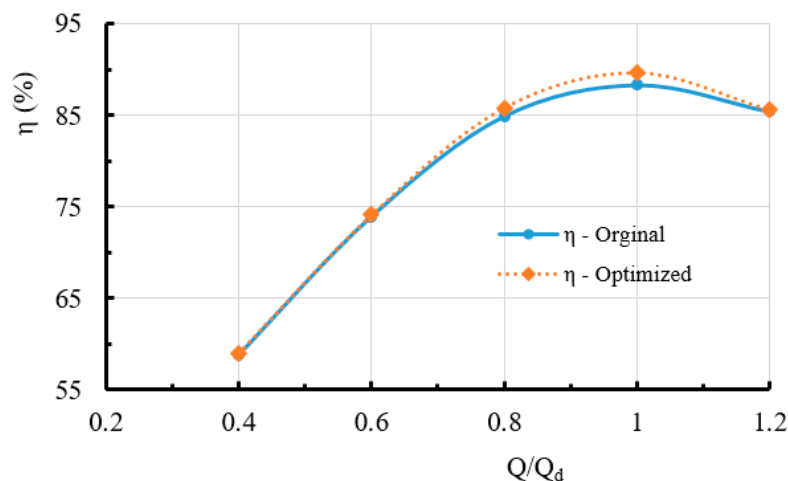
Figure 17. Predicted efficiency comparison at different flow rates.
