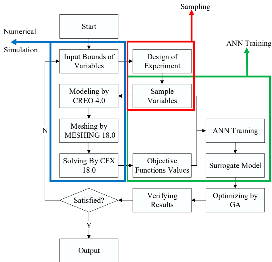
Figure 6. Flowchart of Optimization process.
