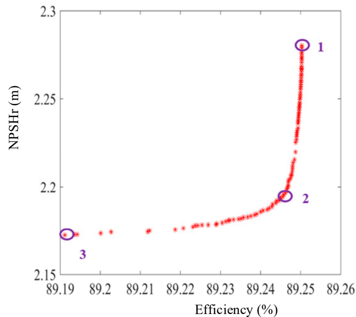
Figure 15. Pareto-frontiers from ANN.
