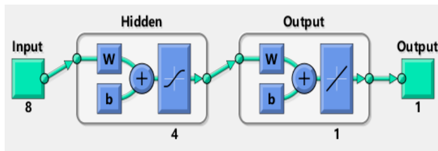
Figure 9. ANN structure for NPSHr objective.
