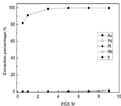
Figure 1. Effect of HCl concentration on the extraction of metals in a HCl solution containing Au(III), Pd(II), Pt(IV), Rh(III), and Ir(IV). ([HCl] = 0.5–9 M, [Cyanex 272] = 0.2 M, O/A = 1, [Au(III)] = [Pd(II)] = [Pt(IV)] = [Rh(III)] = [Ir(IV)] = 100 mg/L).
