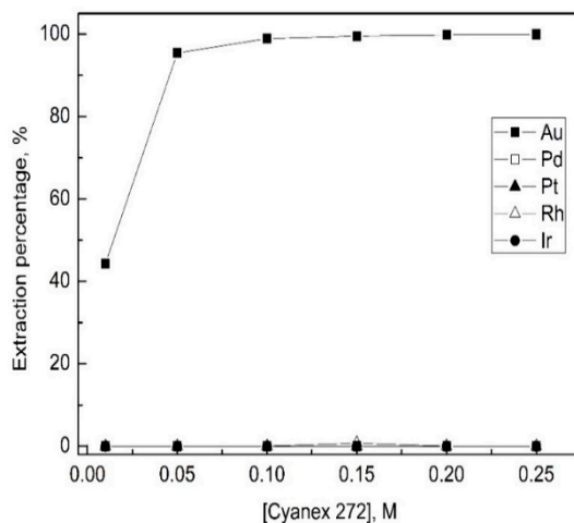
Figure 2. Effect of Cyanex 272 concentration on the extraction of metals containing Au(III), Pd(II), Pt(IV), Rh(III), and Ir(IV). ([HCl] = 5 M, [Au(III)] = [Pd(II)] = [Pt(IV)] = [Rh(III)] = [Ir(IV)] = 100 mg/L).
