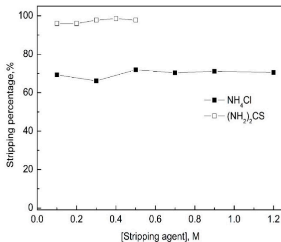
Figure 3. Stripping of Au(III) from the loaded Cyanex 272 by different stripping agents. ((Cyanex 272) = 0.2 M, Loaded (Au(III)) = 99.9 mg/L, ( \text{NH}_4\text{Cl} ) = 0.1–1.2 M, ( (\text{NH}_2)_2\text{CS} ) = 0.1–0.5 M).
