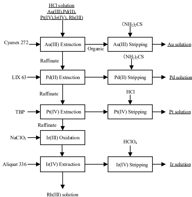
Figure 4. Integrated process for the separation of noble metals from a HCl solution by solvent extraction.
