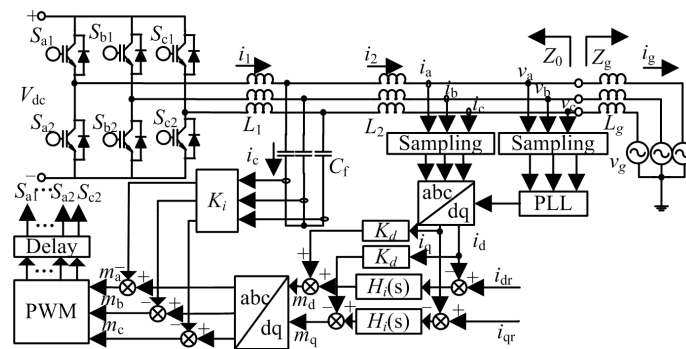
Figure 1. Block diagram of LCL-type inverter with dq -domain GC feedback for grid-connected applications.
