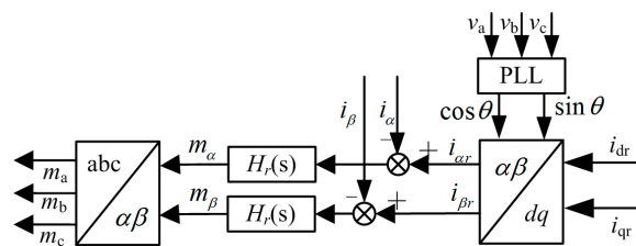
Figure 3. Block diagram of a current controller with \alpha\beta -domain current feedback.
