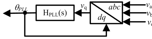
Figure 5. Block diagram of a SRF-PLL.
