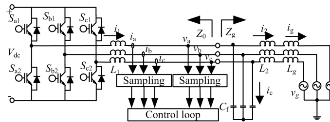
Figure 2. Block diagram of LCL-type inverter with IC feedback.
