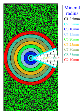
Figure 8. Mineral radii.
