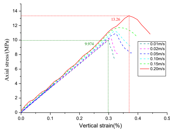
Figure 6. Stress–strain curves under different loading velocities.
