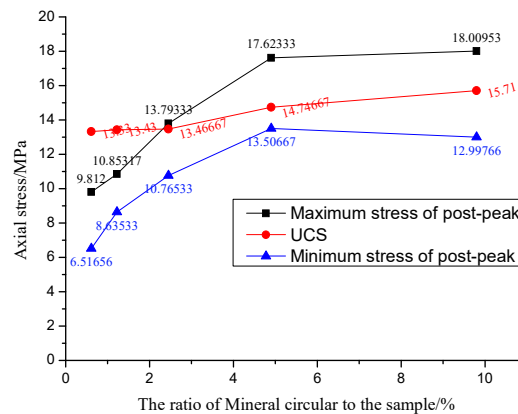
Figure 26. UCS and maximum and minimum stress post-peak for different mineral ratios.
