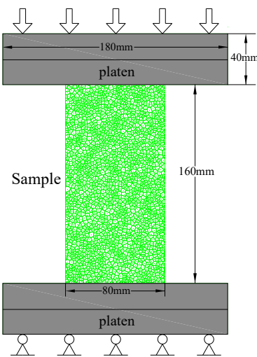
Figure 4. Numerical model of uniaxial compression test.
