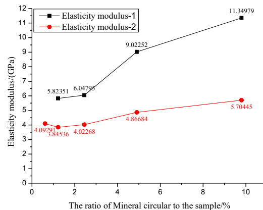
Figure 25. Mean value of elastic modulus for different mineral proportions.
