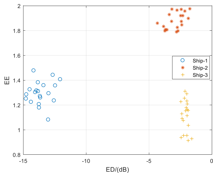
Figure 8. The hybrid feature distribution for S-RN signals.
