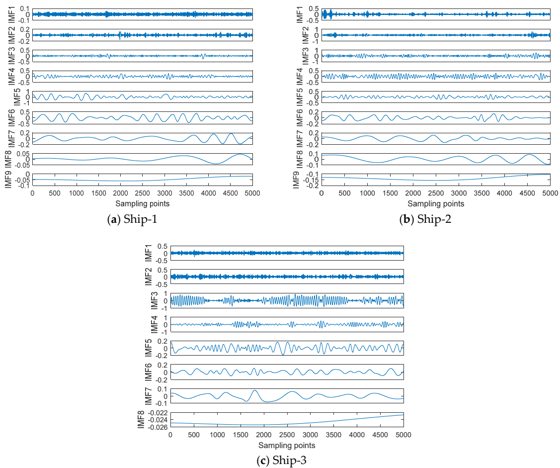
Figure 3. CEEMNAN results for S-RN signals.
