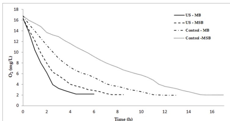
Figure 3. Deoxidation process conducted in malt broth (MB) and molasse broth (MSB) using ultrasound (US). Control: samples without US treatment. The results are arithmetic averages of three independent measurements.
