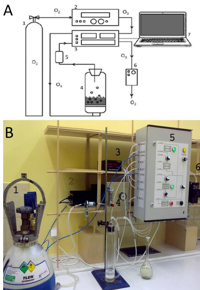
Figure 1. The ozonation system: (A) general scheme; (B) laboratory equipment; 1—oxygen cylinder, 2—ozone generator, 3—ozone analyzer, 4—ozone bubble column, 5—foam trap, 6—residual ozone absorber, 7—computer.
