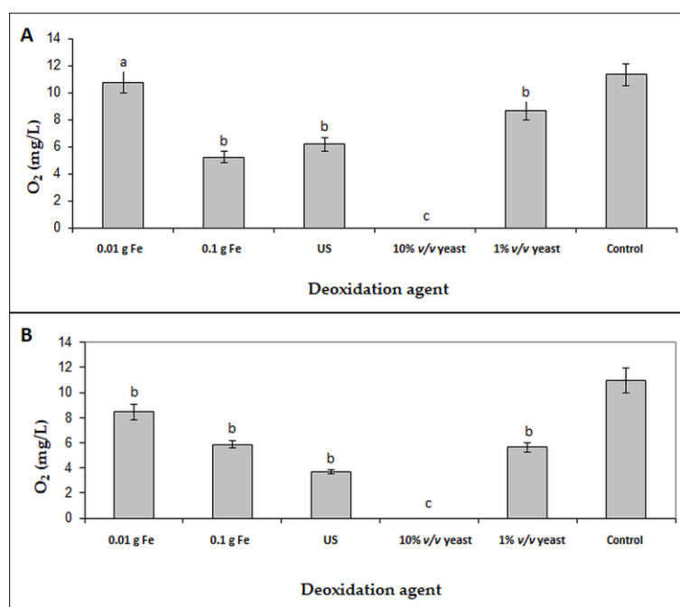
Figure 7. Comparison of oxygen concentration after 2 h of deoxygenation by various methods for MB broth (A) and comparison of oxygen concentration after 4.5 h of deoxygenation by various methods for MSB broth (B). The results were analyzed using one-way repeated measures analysis of variance (ANOVA). Values with different letters are statistically different ( p < 0.05 ). a: p \geq 0.05 ; b: 0.005 < p < 0.05 ; c: p < 0.005 .
