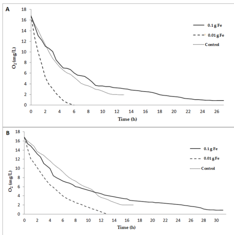
Figure 4. Deoxidation process conducted in MB (A) and MSB (B) broths using FeSO 4 in two doses: 0.1 g/500 mL and 0.01 g/500 mL. Control: samples without FeSO 4 treatment. The results are arithmetic averages of three independent measurements.
