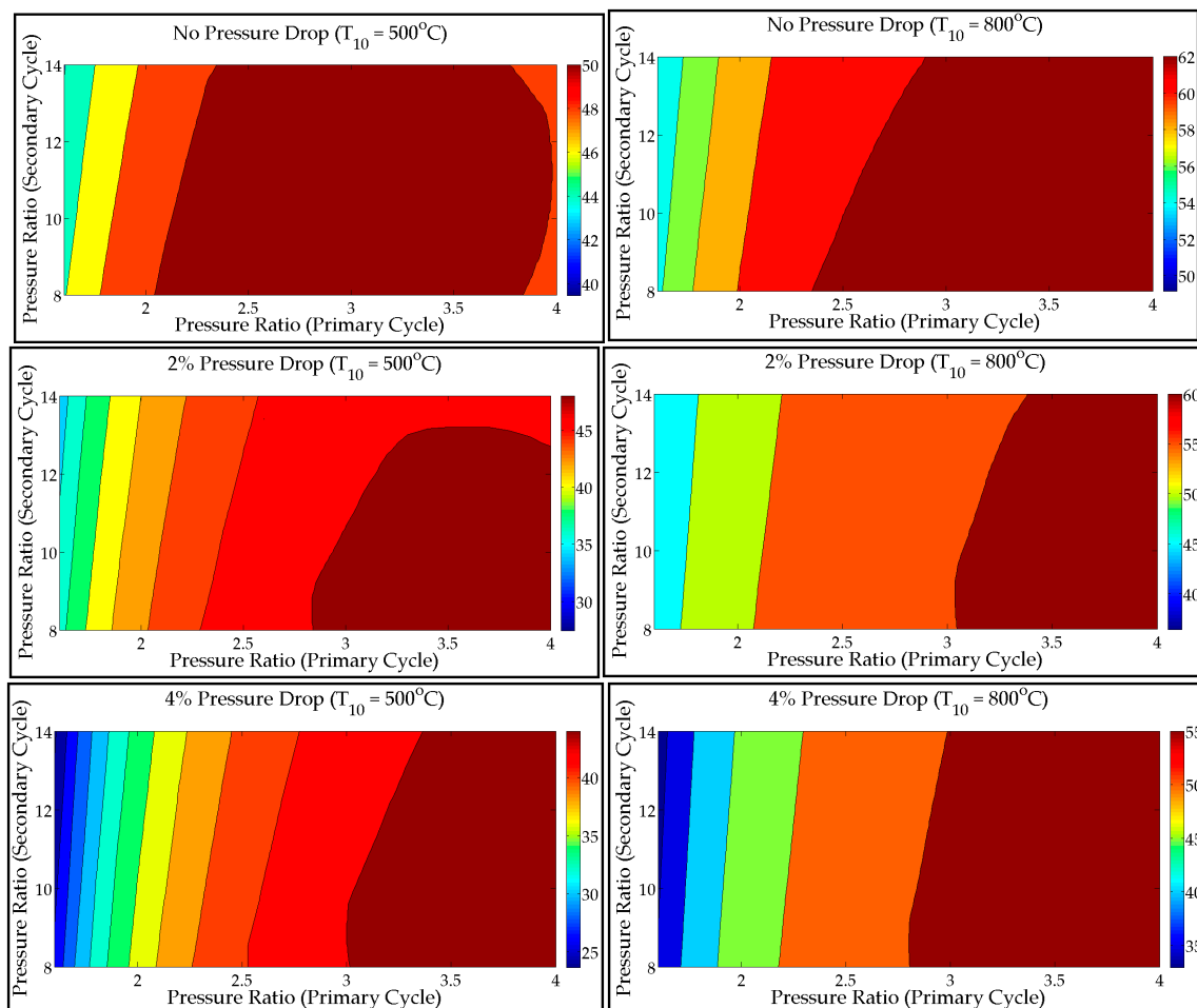
Figure 8. Contour plots of the thermal efficiency of the combined cycle as a function of pressure ratios of the primary and secondary cycles for turbine inlet temperatures of (left) 500 °C and (right) 800 °C in (top) the no-pressure-drop condition, (center) the 2% pressure drop condition, and (bottom) the 4% pressure drop condition. CO 2 is considered as the working fluid in the secondary cycle.
