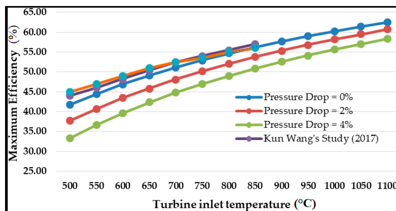
Figure 5. Thermal efficiency of the primary cycle plotted against turbine inlet temperature for the no-pressure-drop, the 2% pressure drop, and the 4% pressure drop conditions. Data points taken from references [32,35] are also plotted for comparison.
