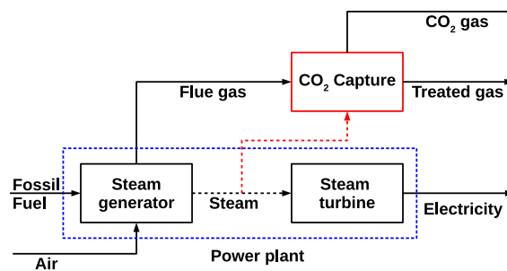
Figure 1. Overview of electricity generation with post-combustion CO 2 capture.
