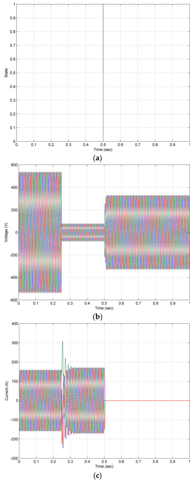
Figure 8. (a) CB10 CLOSE/TRIP state; (b) Feeder voltage waveforms of CB 10 under grid-connected mode and fault occurrence at Bus 1; (c) Feeder current waveforms of CB 10 under grid-connected mode and fault occurrence at Bus 1.
