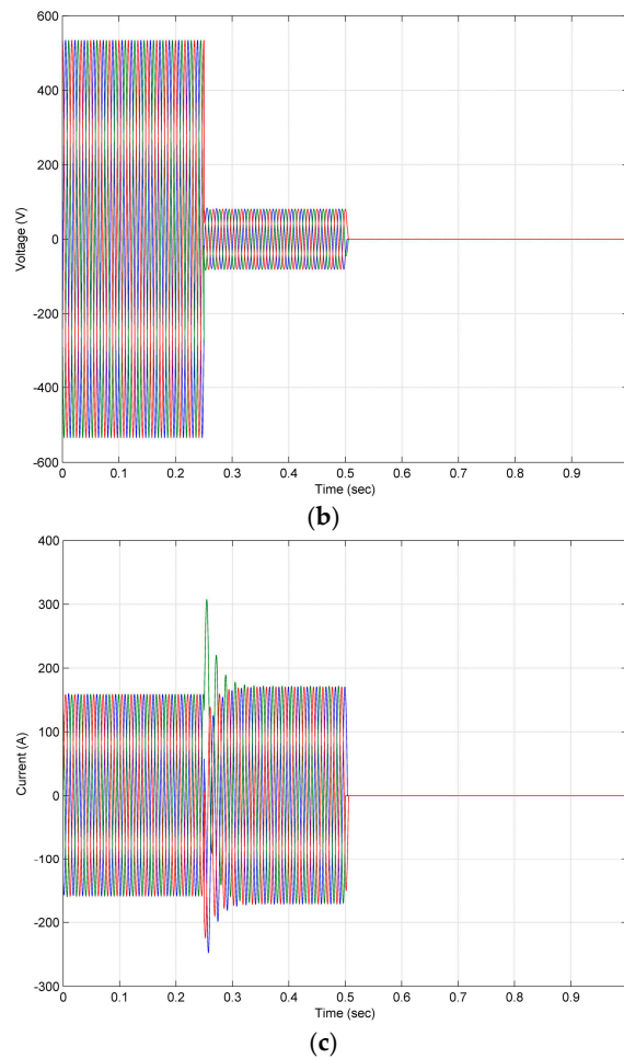
Figure 11. (a) CB11 CLOSE/TRIP state; (b) Feeder voltage waveforms of CB11 under grid-connected mode, fault occurrence at Bus 1 and failure trip of CB10; (c) Feeder current waveforms of CB11 under grid-connected mode, fault occurrence at Bus 1 and failure trip of CB10.
