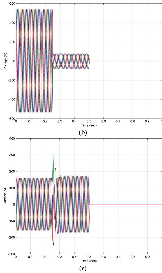
Figure 10. (a) CB10 CLOSE/TRIP state; (b) Feeder voltage waveforms of CB10 under grid-connected mode, fault occurrence at Bus 1 and failure trip of CB10; (c) Feeder current waveforms of CB10 under grid-connected mode, fault occurrence at Bus 1 and failure trip of CB10.
