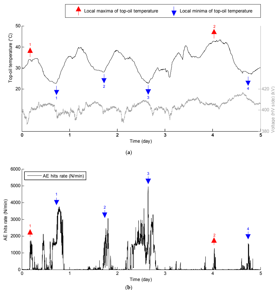
Figure 5. (a) Comparison of voltage, top-oil temperature (peaks and troughs are marked by arrows); and (b) PD activity (AE hits rate per minute) registered in the low voltage LV1 phase during five-day monitoring of a 250 MVA/400 kV/110 kV power transformer.
