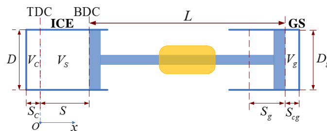
Figure 6. Crucial geometric parameters description of FPLG.
