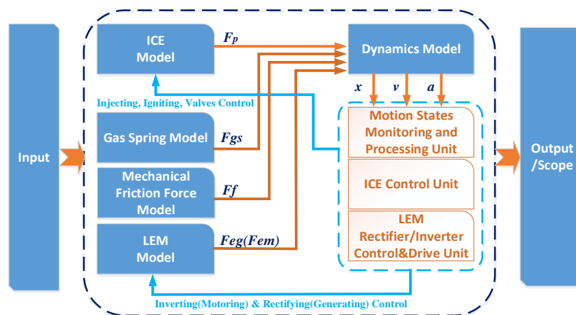
Figure 13. Simulation model diagram.
