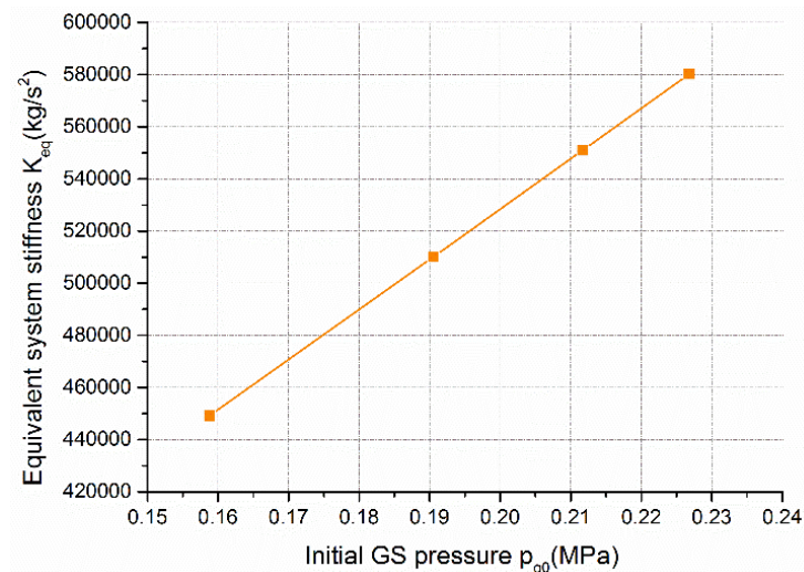
Figure 9. The equivalent system stiffness versus initial GS pressure.
