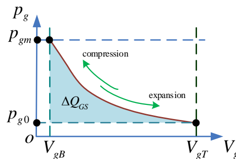
Figure 7. P-V diagram of GS.
