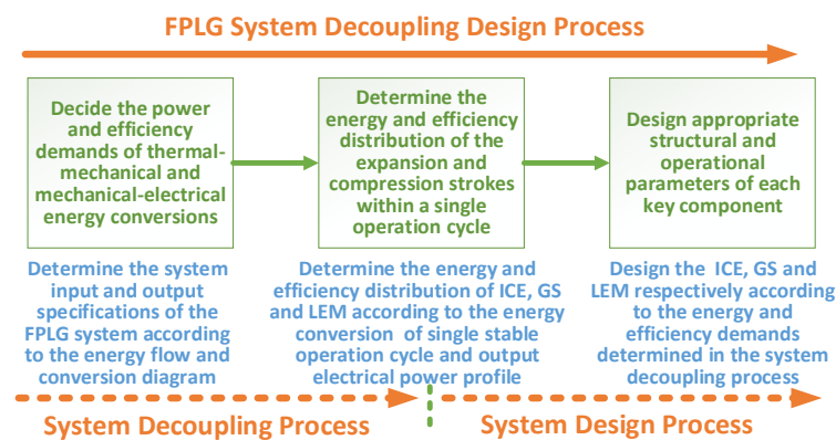
Figure 2. Proposed decoupling design process of FPLG system.
