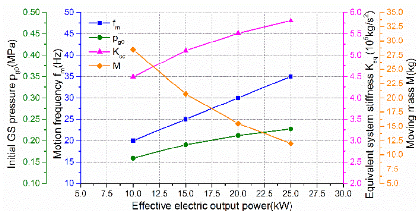
Figure 10. Operational parameters versus effective electric output power map.
