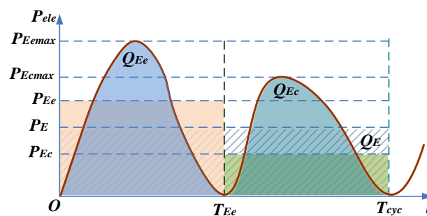
Figure 5. Electric power output of each operation cycle.
