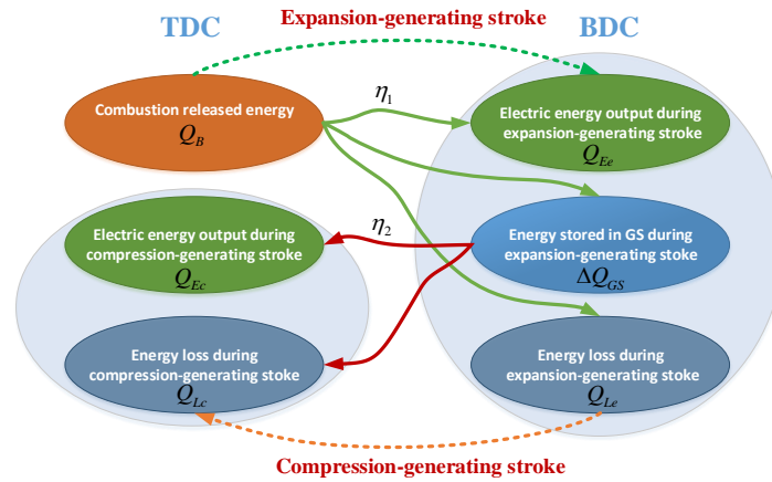
Figure 4. Simplified energy distribution of each operation cycle at stable operation.
