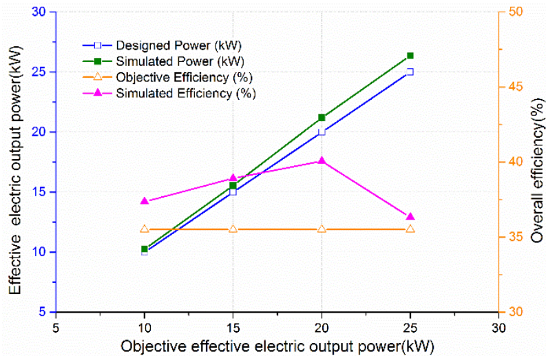
Figure 16. Power and efficiency comparison for various power demands.
