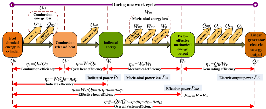
Figure 3. System energy flow diagram.
