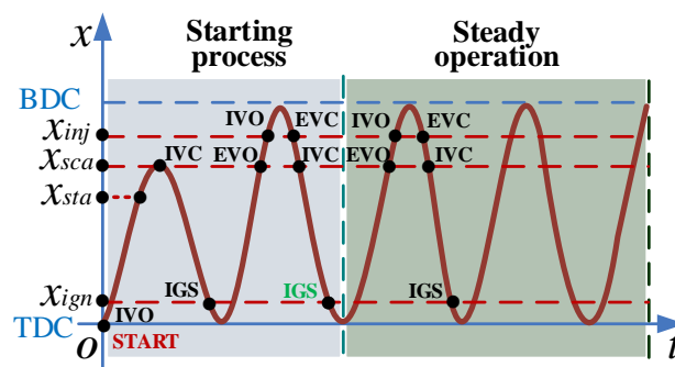
Figure 8. Starting process and steady operation illustration.
