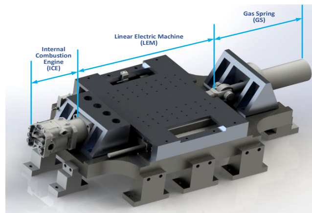
Figure 1. The 3D structure of a FPLG.
