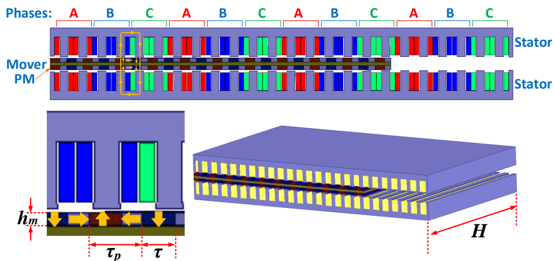
Figure 12. Axial cross-section 2D diagram and flux lines of the PMSLM.
