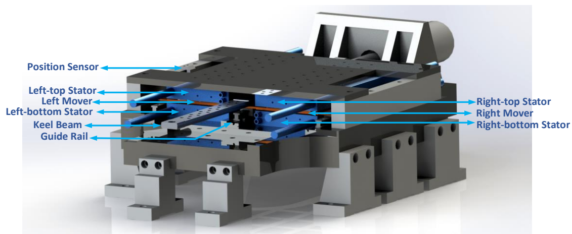
Figure 11. The 3D structure illustration of the linear electric machine.
