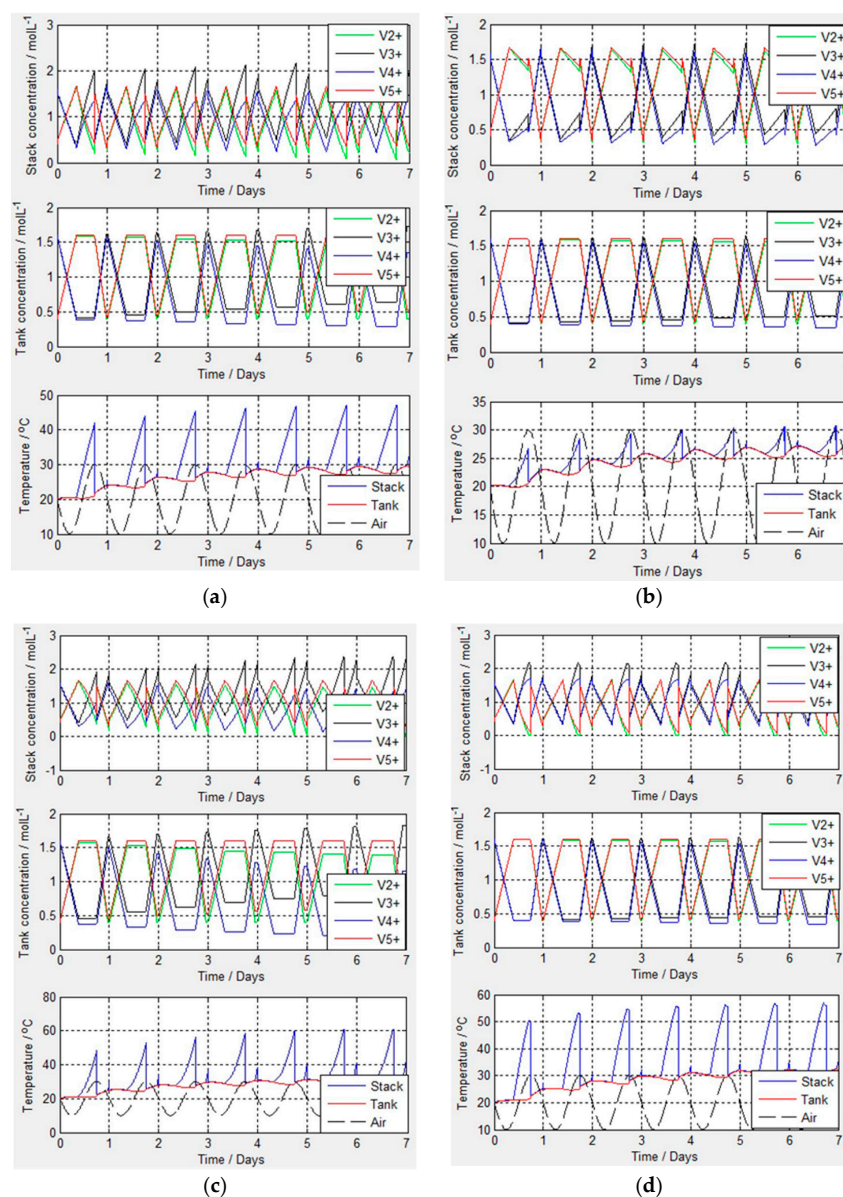
Figure 6. The simulated concentration and temperature variation of (a) FAP450; (b) VB2; (c) F930 and (d) Nafion 115 in a week.
