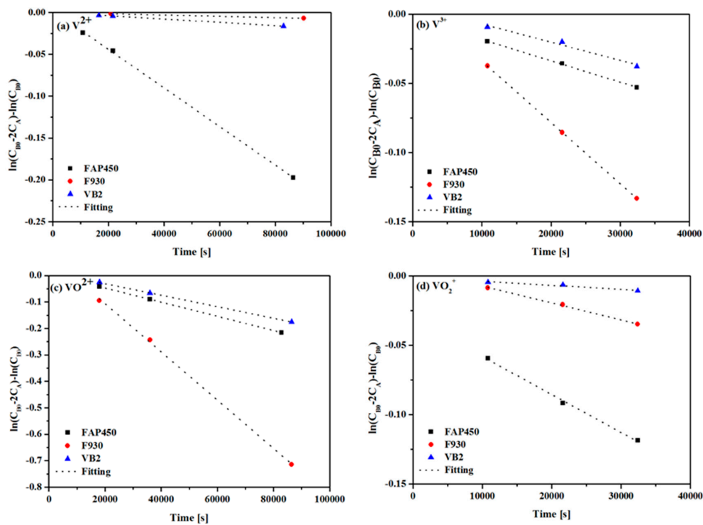
Figure 3. Plot of concentration function vs. time for (a) V^{2+} ; (b) V^{3+} ; (c) VO^{2+} ; and (d) VO_2^+ in the enrichment cell with (■) FAP450, (●) F930 and (▲) VB2 membranes. The dot line is the fitting curve for the data obtained after 180 min.
