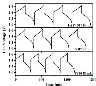
Figure 4. Charge-discharge profiles under constant current charge at 40 \text{ mA} \cdot \text{cm}^{-2} for FAP450, VB2 and F930 membranes.
