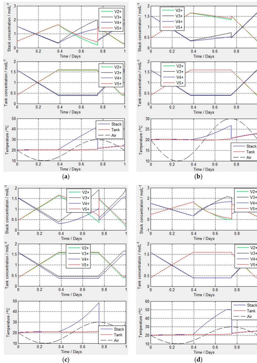
Figure 5. The simulated concentration and temperature variation of (a) FAP450; (b) VB2; (c) F930; and (d) Nafion 115 in the first day.
