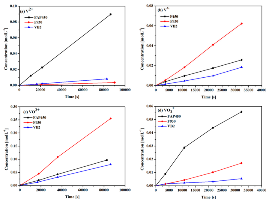
Figure 2. Concentration of vanadium ions: (a) \text{V}^{2+} ; (b) \text{V}^{3+} ; (c) \text{VO}^{2+} ; and (d) \text{VO}_2^+ in the enrichment cell with (■) FAP450, (●) F930 and (▲) VB2 membranes.
