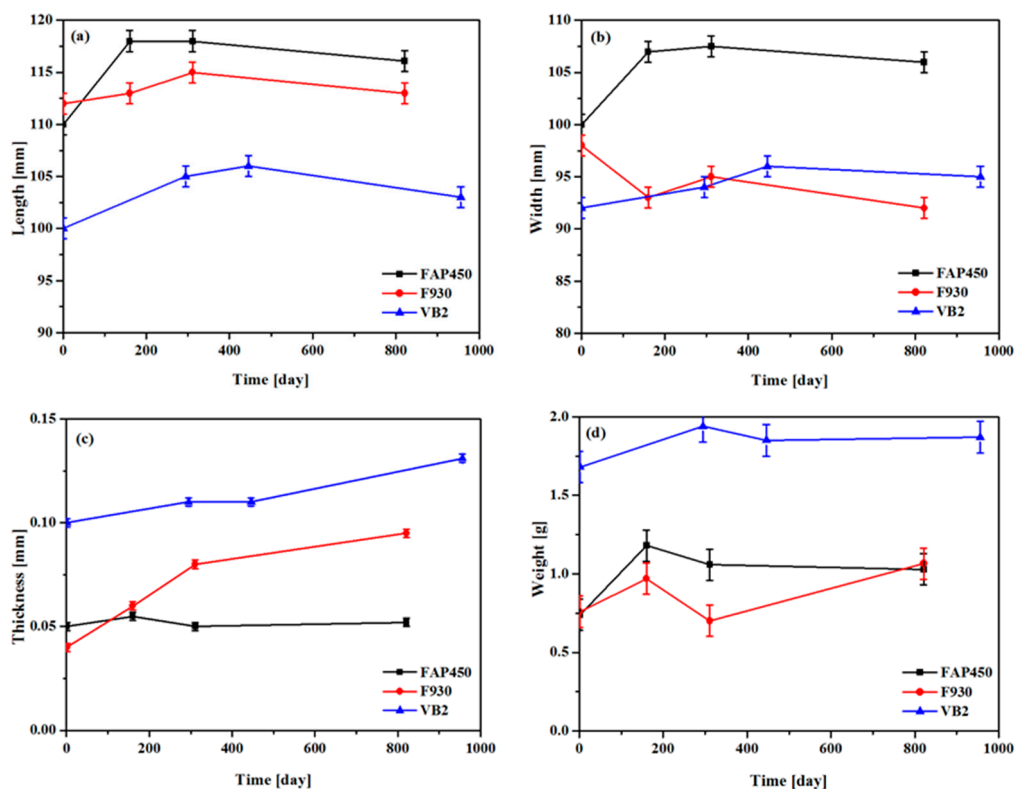
Figure 1. (a) Length; (b) width; (c) thickness; and (d) weight of (■) FAP450, (●) F930 and (▲) VB2 membranes as function of immersing time in 1.6 \text{ mol}\cdot\text{L}^{-1} \text{VO}_2^+ / 4.2 \text{ mol}\cdot\text{L}^{-1} total sulphate solutions.
