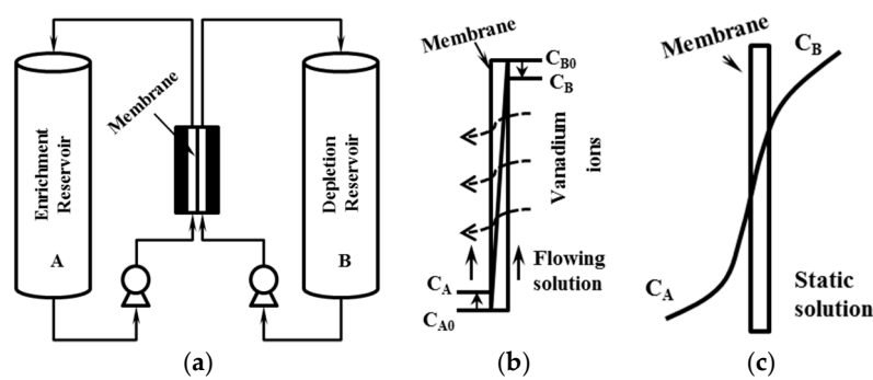
Figure 7. (a) Apparatus for determination of permeability and the concentration gradient; (b) without and (c) with diffusion layer on the surface of membrane.
