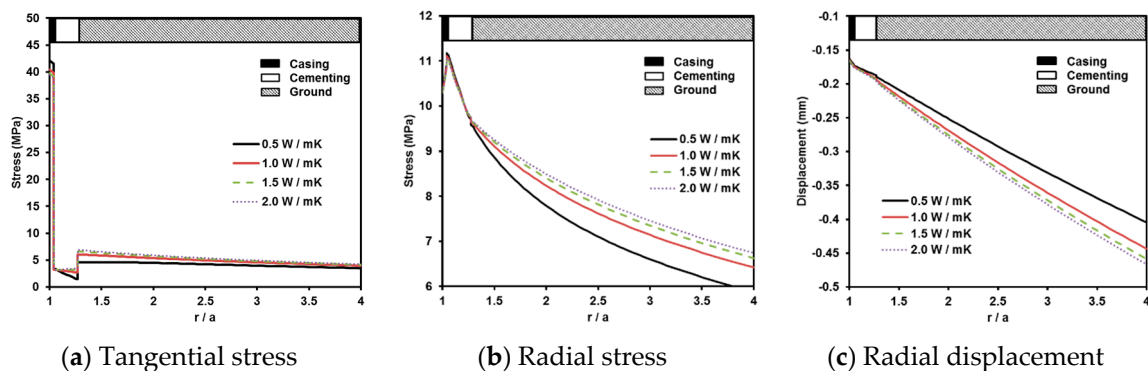
Figure 8. Stress and displacement at 2500 m with variation of thermal conductivity of the cementing component.
