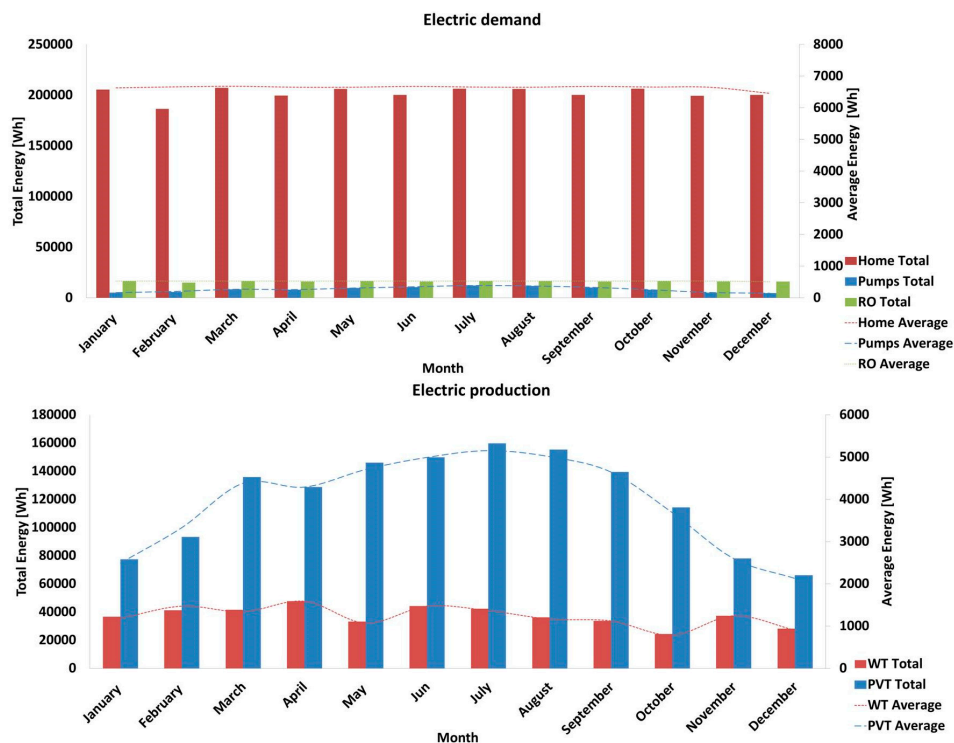
Figure 10. Electric demand and generated power (WT, PVTs).
