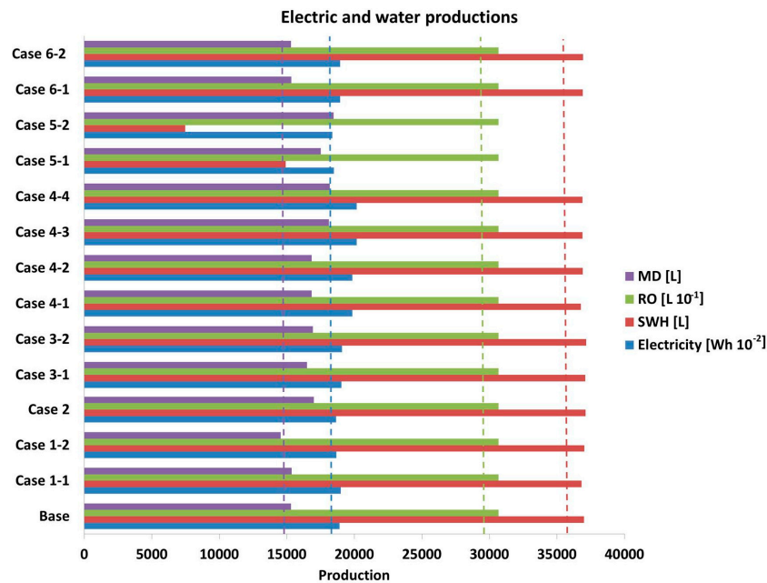
Figure 11. Yearly productions in parametric simulations.
