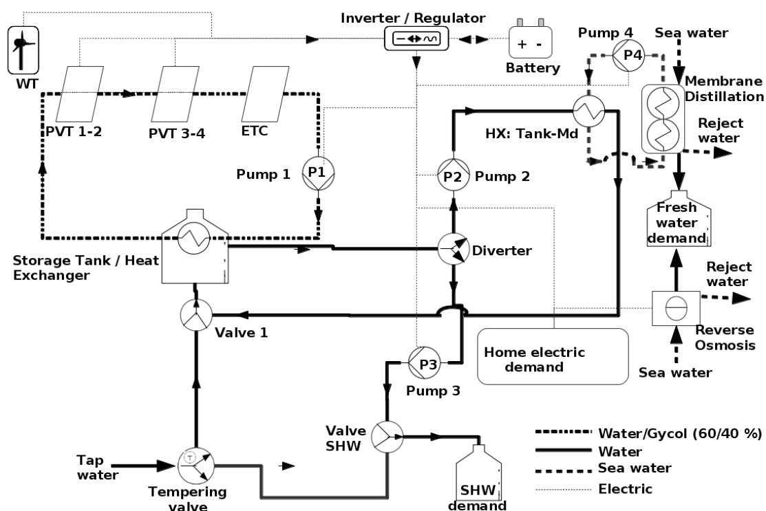
Figure 1. General description of the hybrid trigeneration system.
