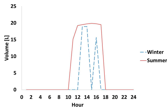
Figure 16. MD production in a typical day per season.
