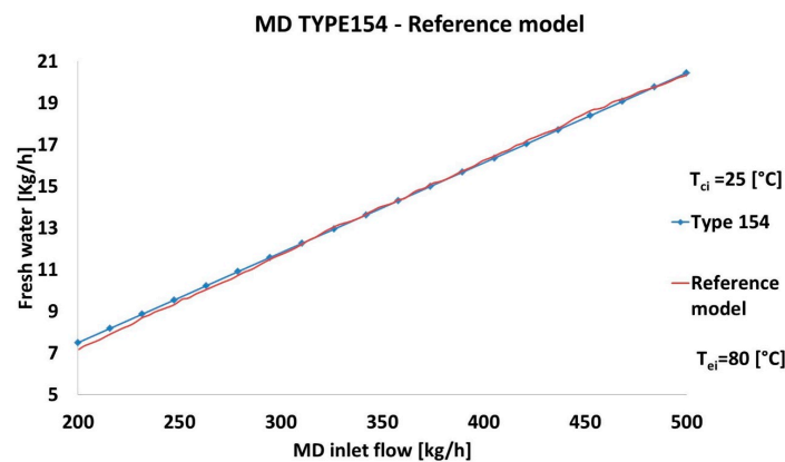
Figure 5. TRNSYS® type and reference model for the PGMD unit (TYPE154 validation).
