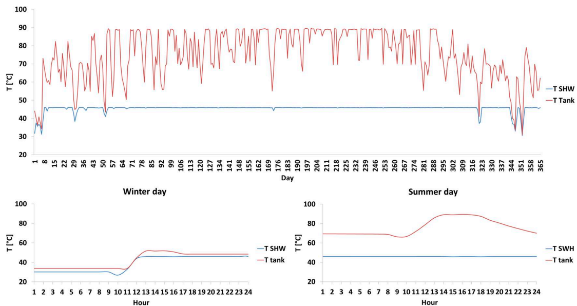
Figure 8. SHW and storage tank temperatures.
