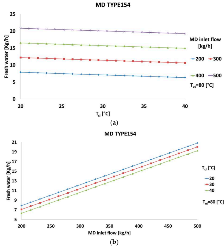
Figure 6. TYPE154 model performance. (a) Condenser inlet temperature effect on fresh water production; (b) Mass inlet flow effect on fresh water production.
