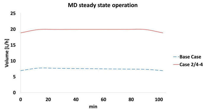
Figure 12. MD distillate at 200 (base case) and 500 L/h (case 2/4-4).
