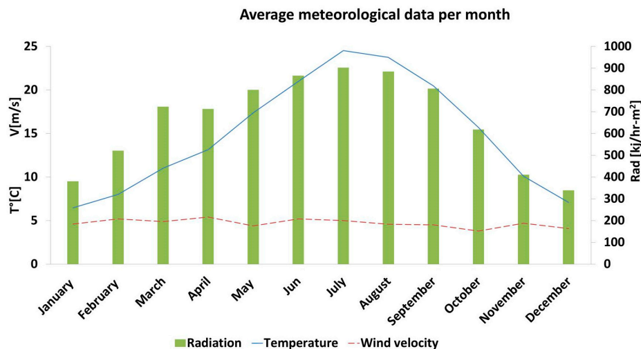
Figure 4. Zaragoza meteorological data.
