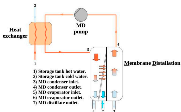
Figure 2. MD basic principle of operation.
