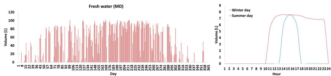
Figure 9. FW production by MD unit along the year.
