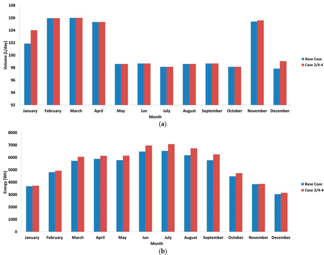
Figure 14. SHW (a) and electricity (b) average production per month.
