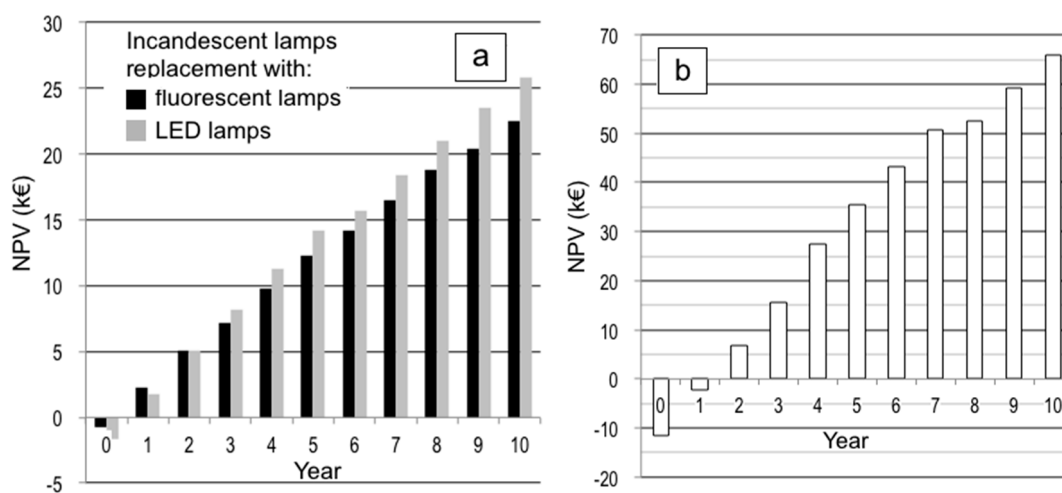
Figure 7. (a) Values of NPV as a function of time in the case of incandescent lamps replacement; and (b) both incandescent and fluorescent lamps replacement.
