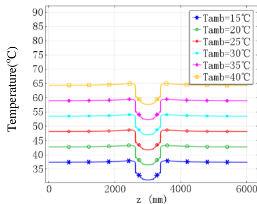
Figure 10. Axial temperature field distribution curves of cable surface with different ambient temperatures.
