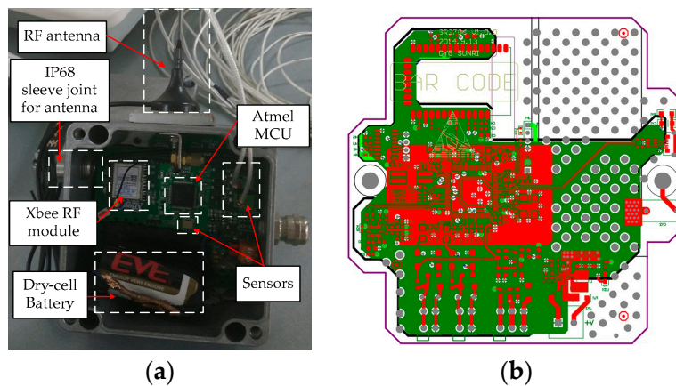
Figure 11. Experimental prototype of wireless sensor devices. (a) wireless sensor node in shell; and (b) and printed circuit board (PCB) design of wireless sensor module.
