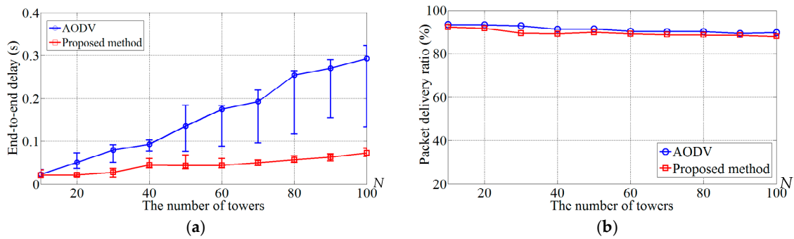
Figure 9. Routing Protocol performance different network scale. (a) average, maximum and minimum end-to-end delay; and (b) packet delivery ratio.
