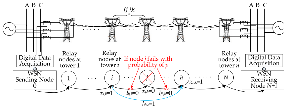
Figure 3. Description of reconstructed communication channel (RCC) model by hop-by-hop relaying.
