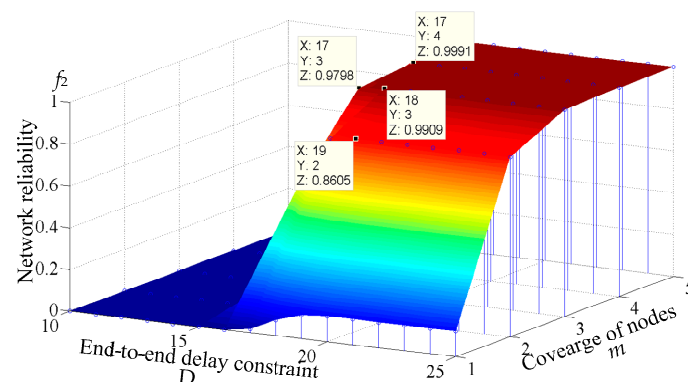
Figure 8. Effect of end-to-end delay constraint.
