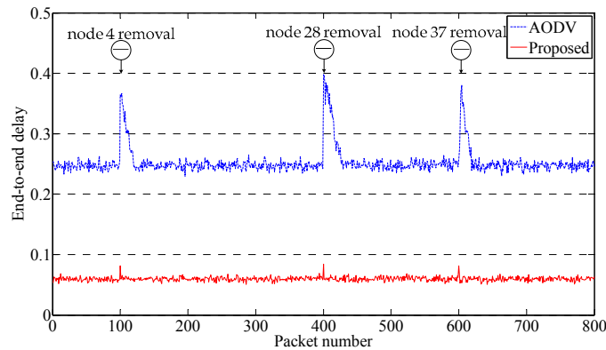
Figure 10. Routing protocol performance with node removal.
