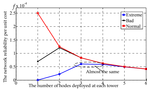
Figure 6. Effect of the number of nodes deployed at each tower.
