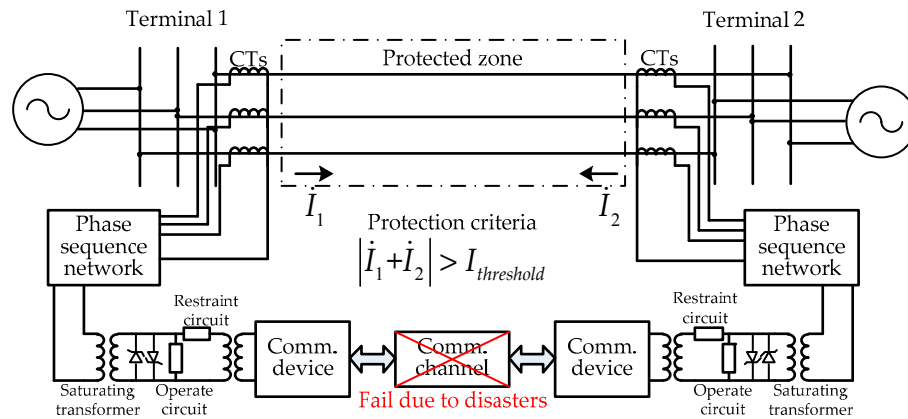
Figure 1. Functional setup of current differential protection.
