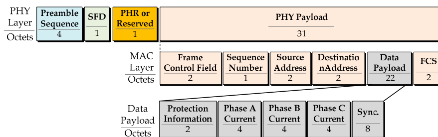
Figure 4. WSN data packet frame.
