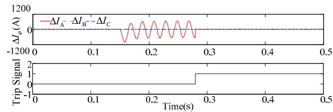
Figure 12. Differential current of each phase and the trip signal (single-phase-to-ground fault happens at 0.16 s).
