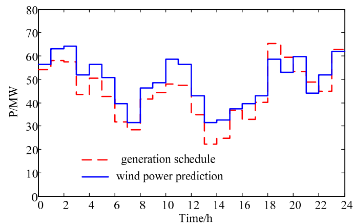
Figure 2. Day-ahead wind power prediction and the generation schedule of integrated system.
