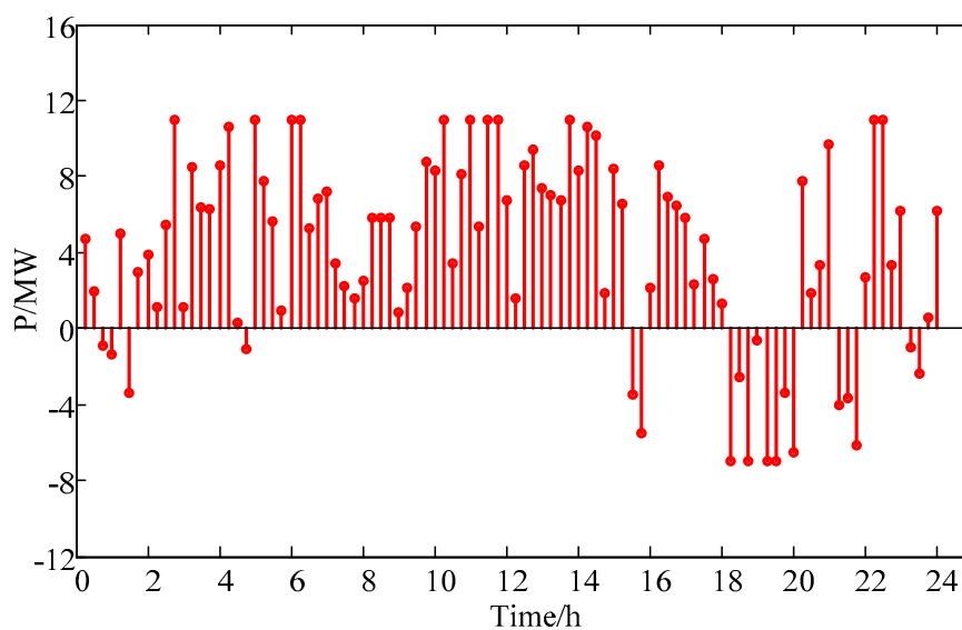
Figure 11. Charging/discharging power of the BSS.
