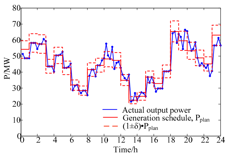
Figure 9. Actual output power of the integrated system.
