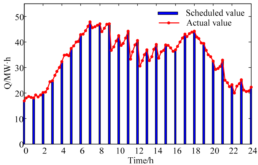
Figure 10. Actual stored energy of the BSS.
