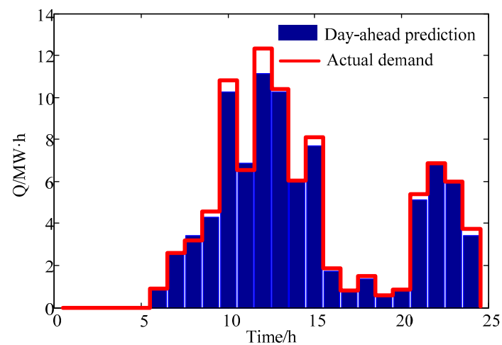
Figure 6. Actual battery swapping demand.
