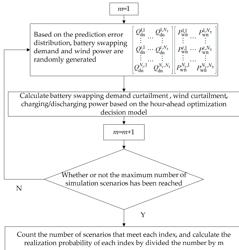
Figure 1. Flowchart of the stochastic simulation.
