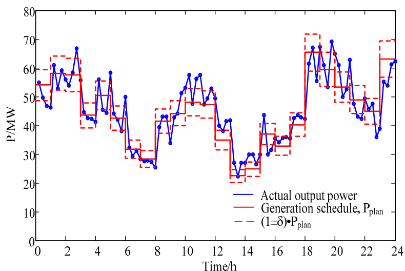
Figure 13. Actual output power of the integrated system in model without considering charging/discharging power readjustment.
