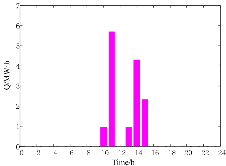
Figure 12. Wind curtailment in model without considering charging/discharging power readjustment.
