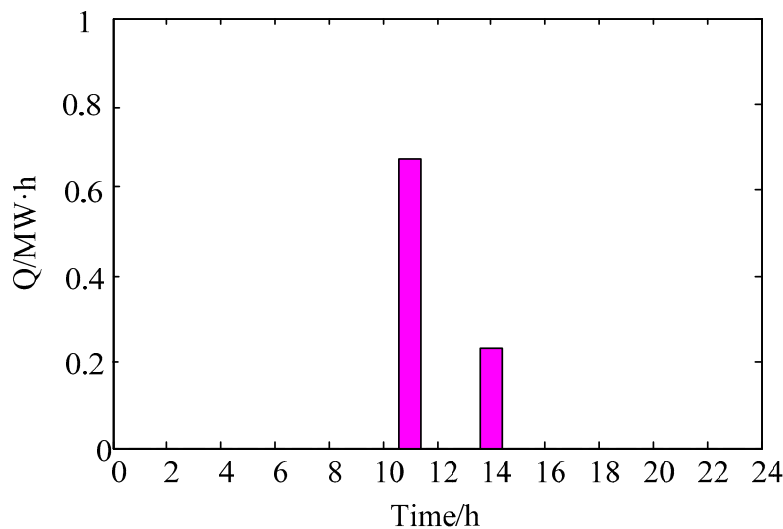
Figure 8. Wind curtailment at each time interval.
