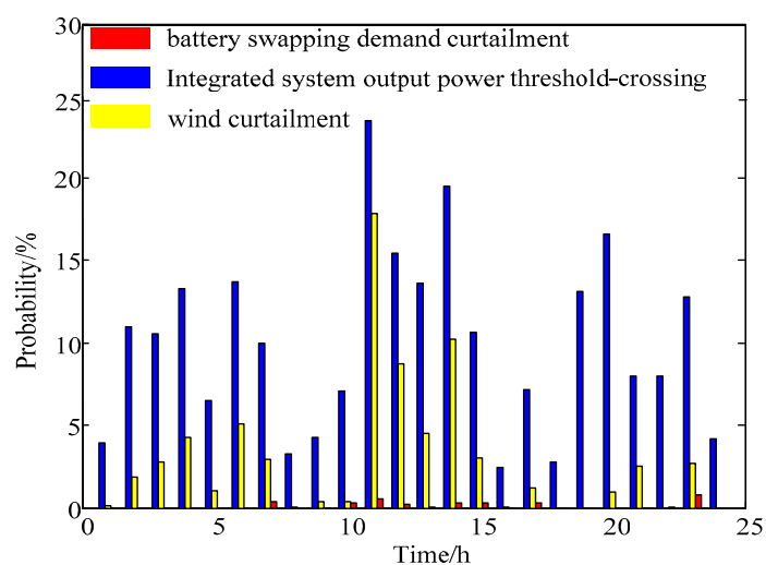
Figure 5. Probabilities for battery swapping demand curtailment, wind curtailment and integrated system output power threshold-crossing.
