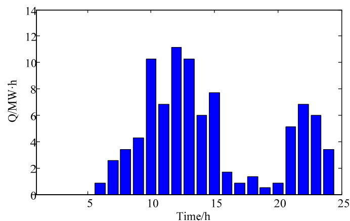
Figure 3. Day-ahead battery swapping demand prediction.
