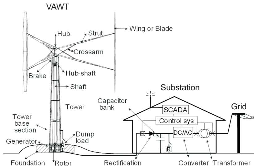
Figure 3. Converter system for the 200 kW VAWT.
