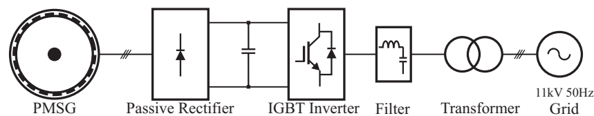
Figure 6. Converter system for the 200 kW VAWT.
