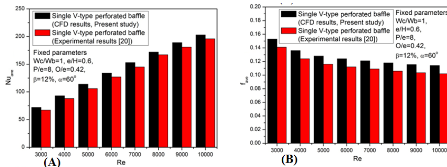
Figure 5. Comparison of experimental results with CFD results of single V-type perforated baffle: (A) Nu_{ave} and (B) f_{ave} .
