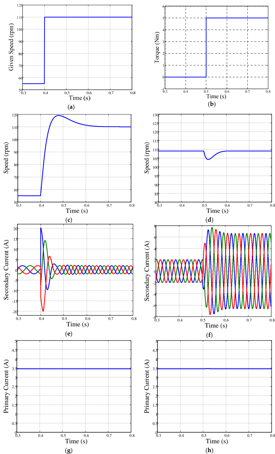
Figure 9. Simulation results of the DC excitation control for the DSFM motor: (a) curve of the given speed variation; (b) curve of the load torque variation; (c) speed curve for speed varying from 55 to 110 rpm; (d) speed curve for torque varying from 0 to 5 Nm; (e) secondary current curve for speed varying from 55 to 110 rpm; (f) secondary current curve for torque varying from 0 to 5 Nm; (g) primary current curve for speed varying from 55 to 110 rpm; and (h) primary current curve for torque varying from 0 to 5 Nm.
