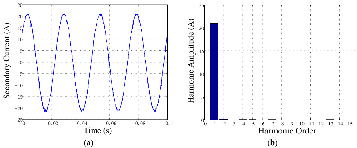
Figure 11. Winding currents of the DSFM motor at 200 rpm: (a) secondary winding current; and (b) the harmonic content of the current.
