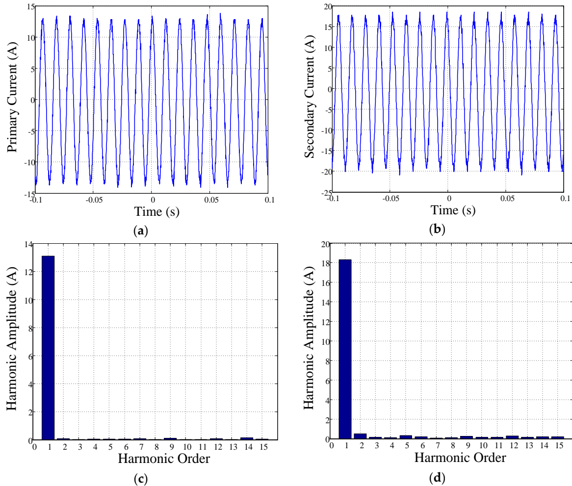
Figure 16. Winding currents of the DSFM motor at 924 rpm: (a) primary winding current; (b) secondary winding current; (c) the harmonic content of the primary current; and (d) the harmonic content of the secondary current.
