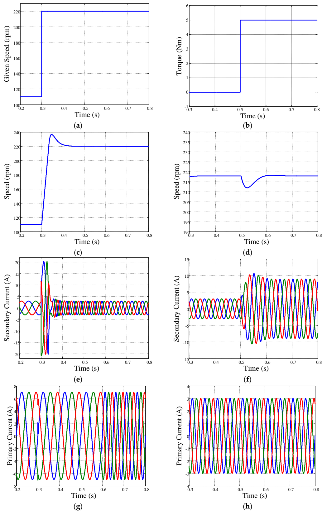
Figure 15. Simulation results of the AC excitation control for the DSFM motor: (a) curve of the given speed variation. (b) curve of the load torque variation; (c) speed curve for speed varying from 110 to 220 rpm; (d) speed curve for torque varying from 0 to 5 Nm; (e) secondary current curve for speed varying from 110 to 220 rpm; (f) secondary current curve for torque varying from 0 to 5 Nm; (g) primary current curve for speed varying from 110 to 220 rpm; and (h) primary current curve for torque varying from 0 to 5 Nm.
