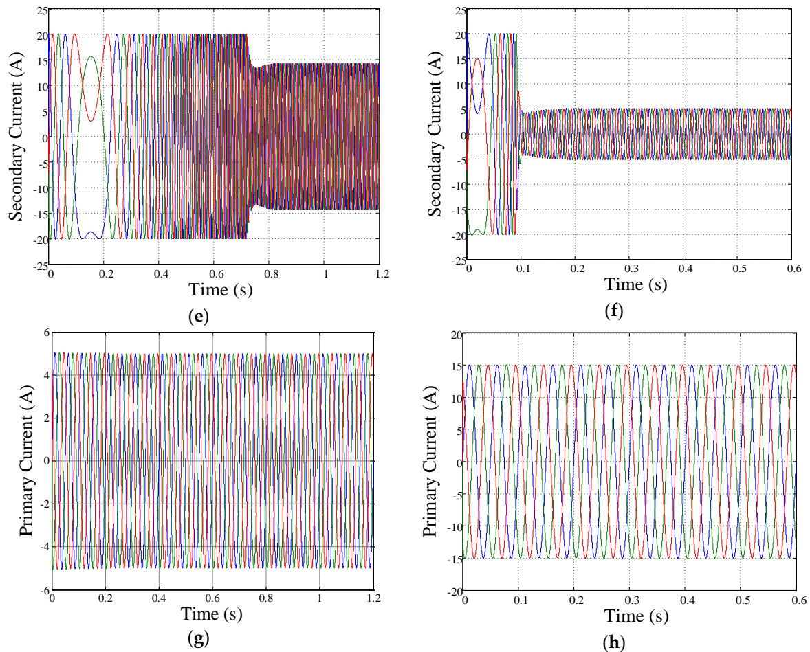
Figure 14. Simulation results of the start-up of the motor under load: (a) speed curve for i_{pd}^* = 5 A; (b) speed curve for i_{pd}^* = 15 A; (c) torque curve for i_{pd}^* = 5 A; (d) torque curve for i_{pd}^* = 15 A; (e) secondary current curve for i_{pd}^* = 5 A; (f) secondary current curve for i_{pd}^* = 15 A; (g) primary current curve for i_{pd}^* = 5 A; and (h) primary current curve for i_{pd}^* = 15 A.
