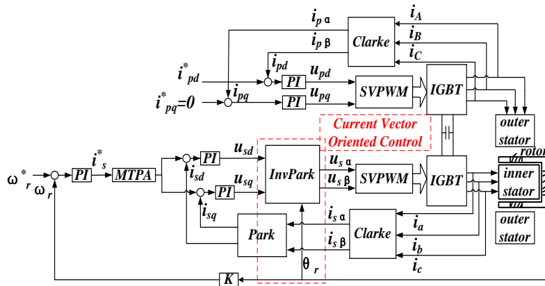
Figure 8. DC excitation control method.
