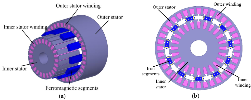
Figure 1. Structure of the DSFM motor with an iron segment rotor: (a) 3D model; and (b) 2D model.
