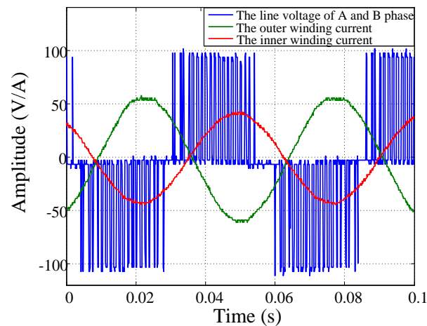
Figure 6. Experimental results of the VVVF control.
