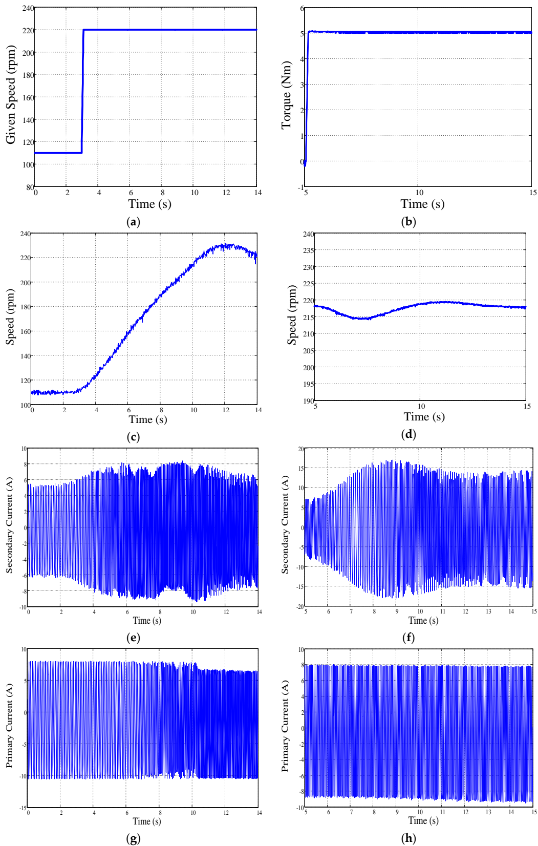
Figure 17. Experimental results of the AC excitation control for the DSFM motor: (a) curve of the given speed variation. (b) curve of the load torque variation; (c) speed curve for speed varying from 110 to 220 rpm; (d) speed curve for torque varying from 0 to 5 Nm; (e) secondary current curve for speed varying from 110 to 220 rpm; (f) secondary current curve for torque varying from 0 to 5 Nm; (g) primary current curve for speed varying from 110 to 220 rpm; and (h) primary current curve for torque varying from 0 to 5 Nm.
