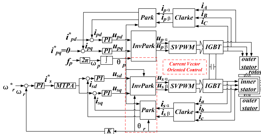
Figure 13. AC excitation control method.
