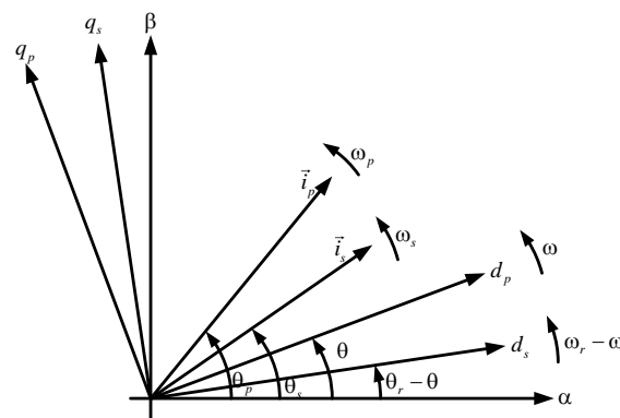
Figure 7. Reference frames and current vectors used in DSFM motor equations.
