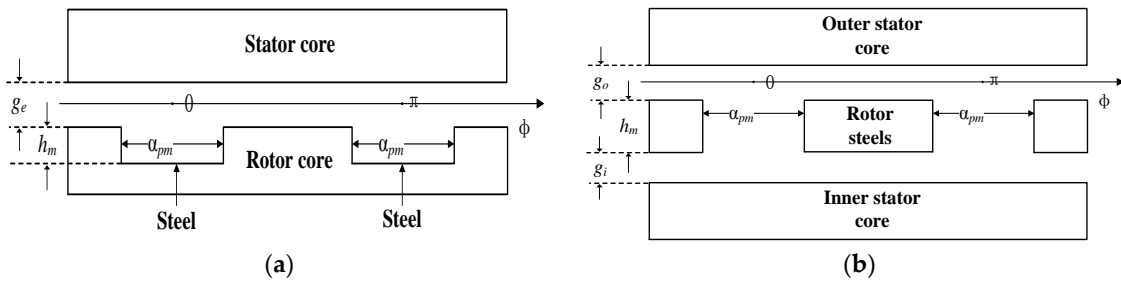
Figure 3. Air gap structures of the (a) BDFRM motor and (b) DSFM motor.
