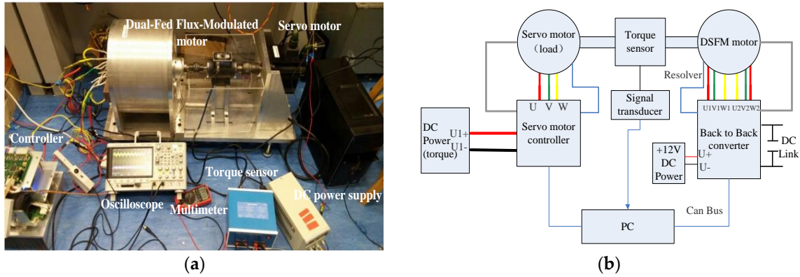
Figure 10. Experimental environment of the DSFM motor: (a) laboratory test facility; and (b) block diagram of the DSFM motor experimental setup.
