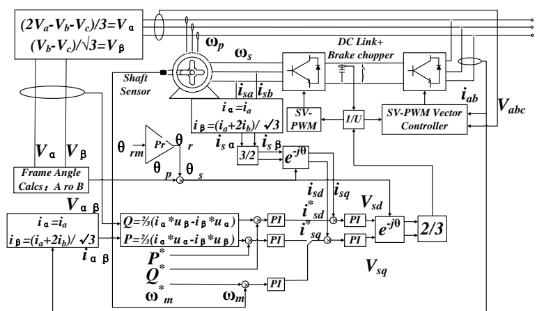
Figure 2. A structural diagram of the BDFRM (G) drive setup.
