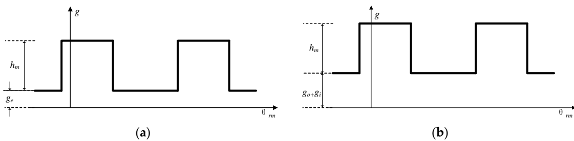
Figure 4. Air gap function of the (a) BDFRM motor and (b) DSFM motor.
