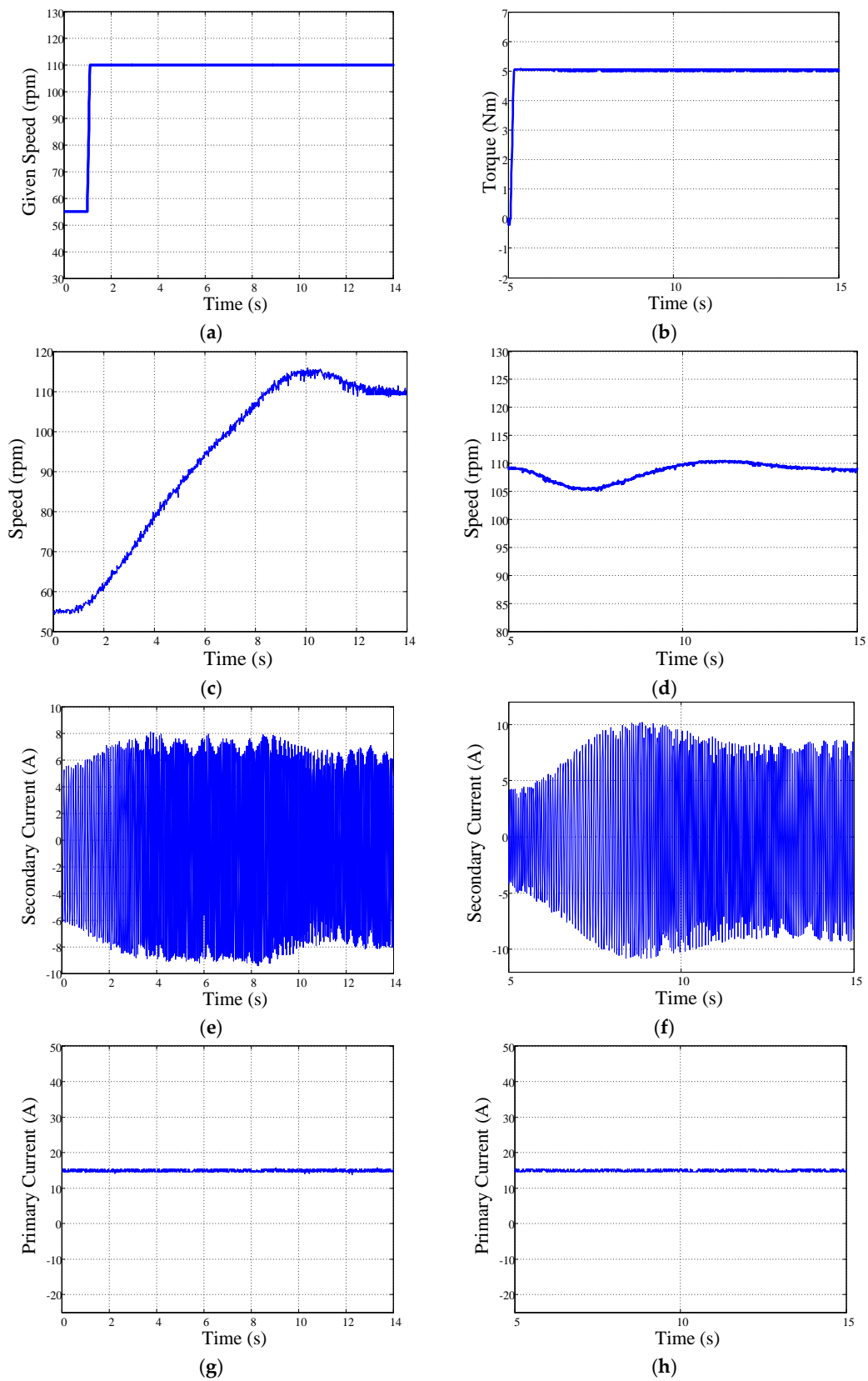
Figure 12. Experimental results of the DC excitation control for the DSFM motor: (a) curve of the given speed variation; (b) curve of the load torque variation; (c) speed curve for speed varying from 55 to 110 rpm; (d) speed curve for torque varying from 0 to 5 Nm; (e) secondary current curve for speed varying from 55 to 110 rpm; (f) secondary current curve for torque varying from 0 to 5 Nm; (g) primary current curve for speed varying from 55 to 110 rpm; and (h) primary current curve for torque varying from 0 to 5 Nm.
