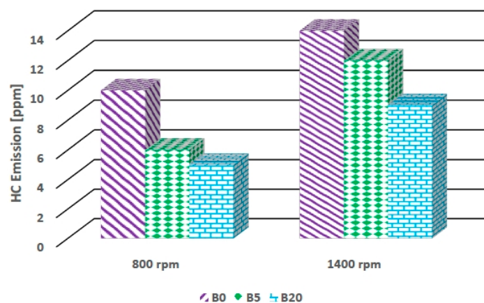
Figure 9. Variation of hydrocarbon emission with speeds.
