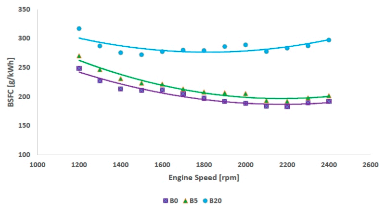
Figure 7. Variation of brake specific fuel consumption with speeds.
