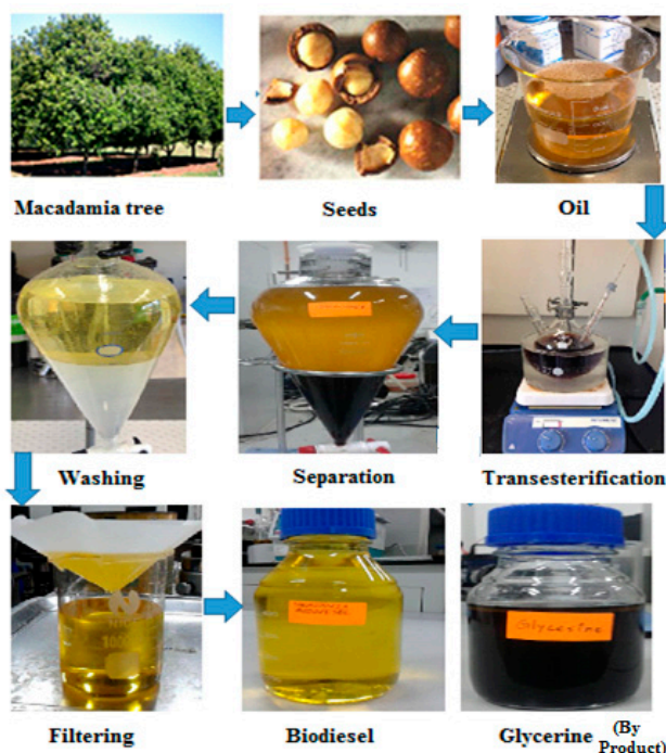
Figure 1. Production of macadamia biodiesel.
