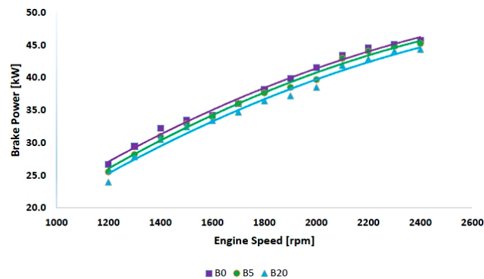
Figure 6. Variation of brake power with speeds.
