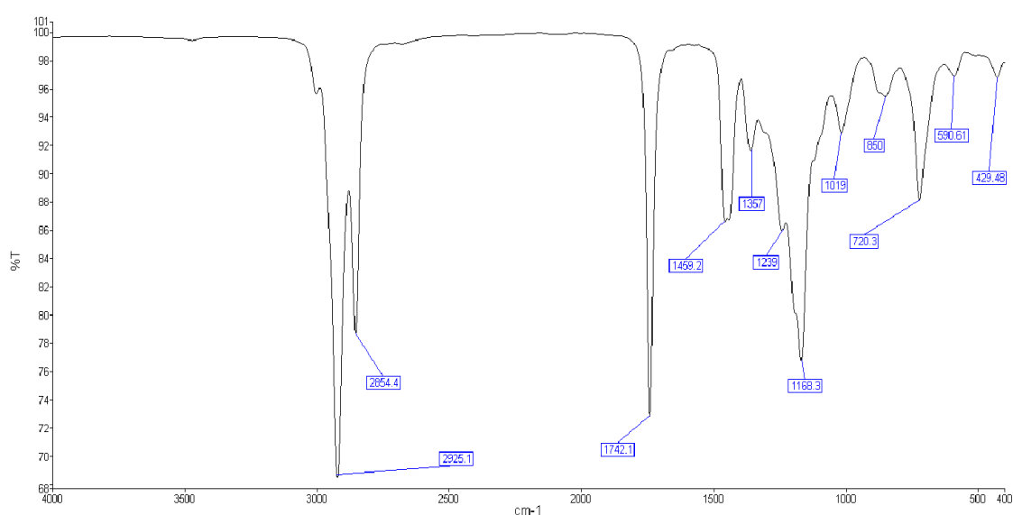
Figure 4. Fourier transform infrared (FT-IR) Spectrum of macadamia biodiesel.
