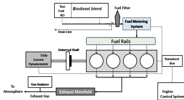
Figure 3. Schematic diagram of the engine test bed.
