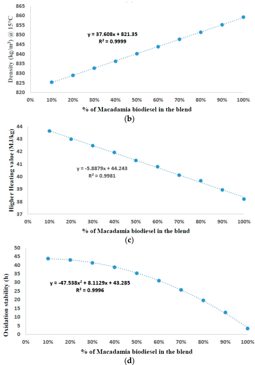
Figure 5. Effect of macadamia biodiesel–diesel blending on (a) KV ; (b) D ; (c) higher heating value ( HHV ); and (d) OS .
