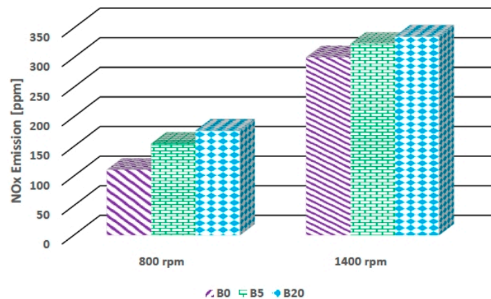
Figure 10. Variation of nitrogen oxides emission with speeds.
