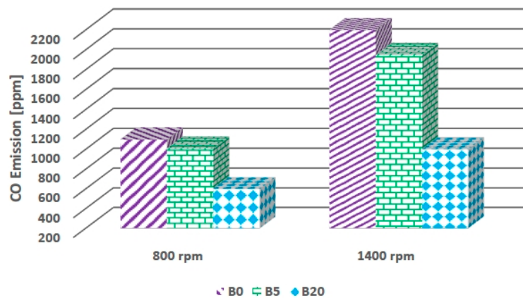
Figure 8. Variation of carbon monoxides emission with speeds.
