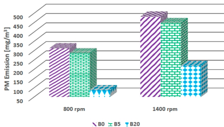
Figure 11. Variation of particulate matter emission with speeds.
