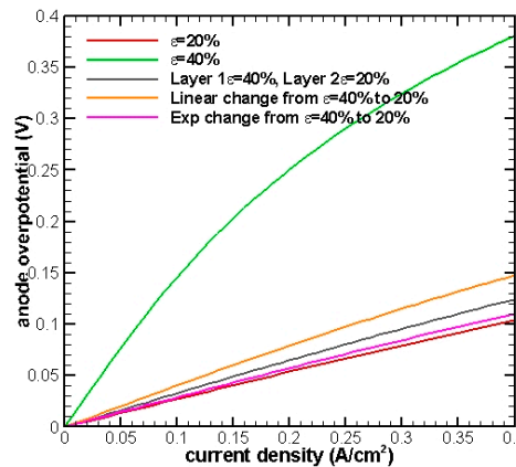
Figure 2. I-V curve for 30- \mu\text{m} anode thickness.
