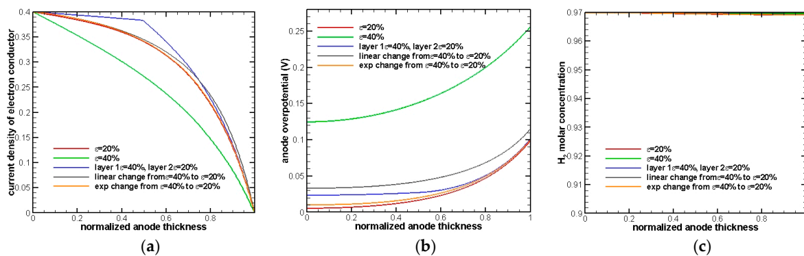
Figure 3. Detailed plots for anode thickness = 30 \mu\text{m} and current density = 0.4 A/cm 2 : (a) distribution of current density in electron conductor; (b) distribution of anode overpotential; and (c) distribution of H 2 molar concentration.
