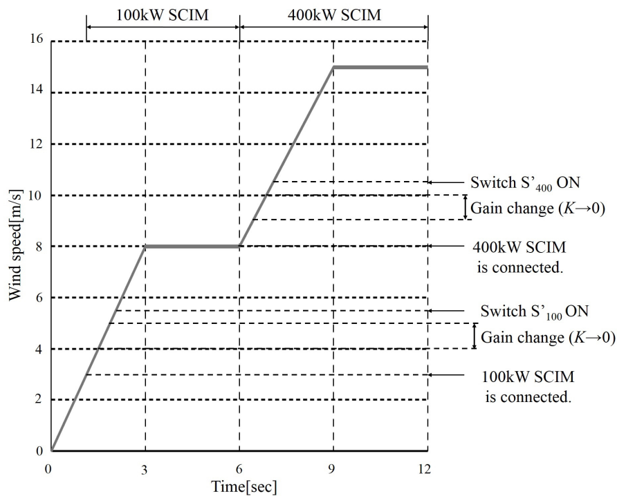
Figure 3. Simulation condition by the wind speed.
