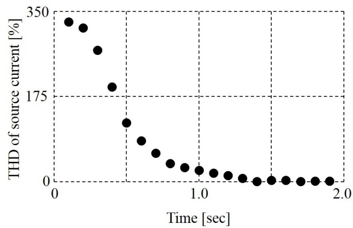
Figure 8. Source current total harmonic distortion (THD) of the soft-starter for the 100-kW SCIM in Figure 7.
