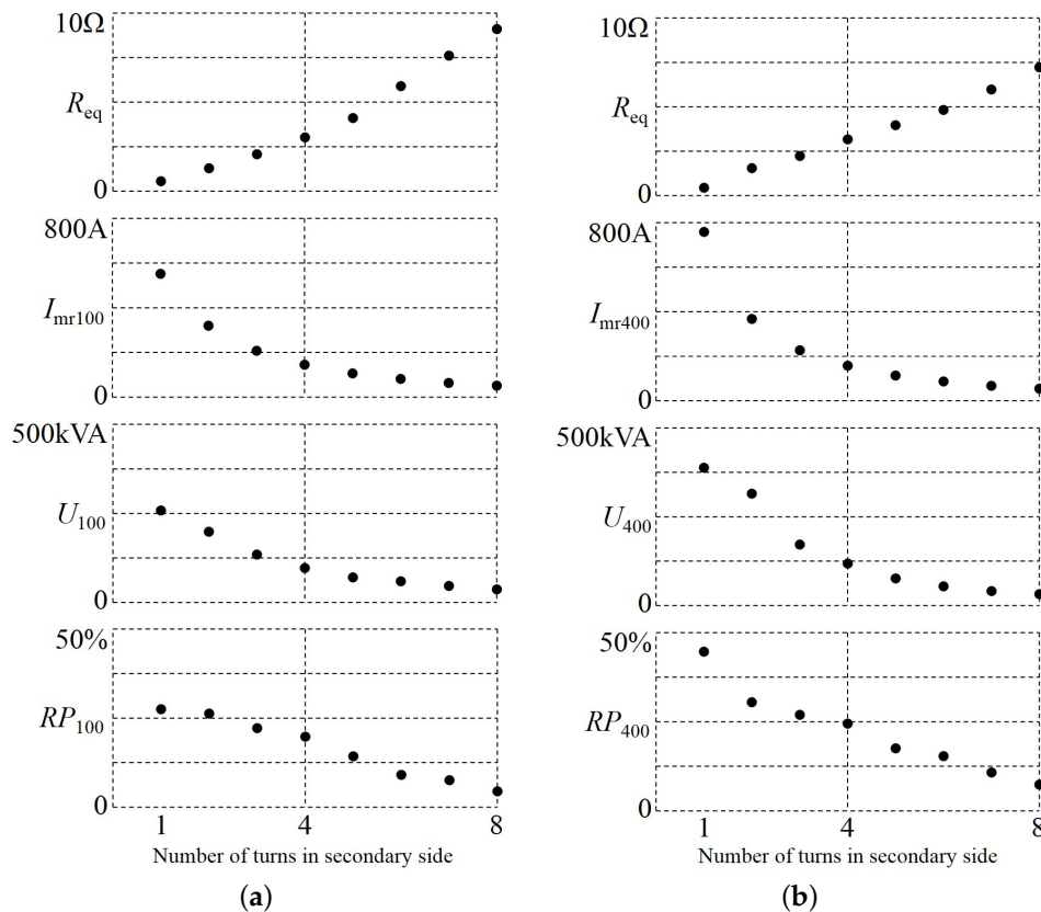
Figure 16. Relationship between the number of turns on the secondary side of the matching transformer and the proposed inrush current suppressor. (a) For the 100-kW SCIM; (b) For the 400-kW SCIM.
