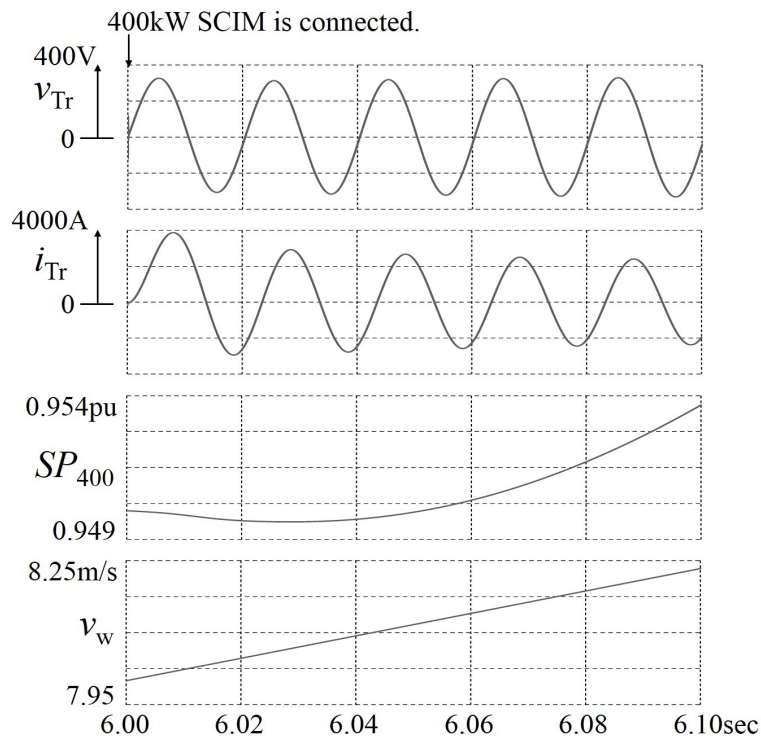
Figure 5. Simulated waveforms of the direct connection for the 400-kW SCIM.
