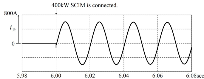
Figure 13. Source current for the 400-kW SCIM with the external resistors.
