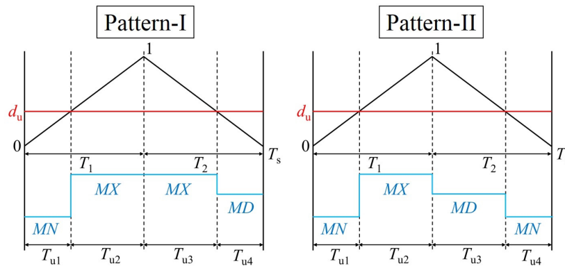
Figure 2. Switching states in Pattern I and Pattern II in the direct duty ratio pulse width modulation (DDRPWM) method.
