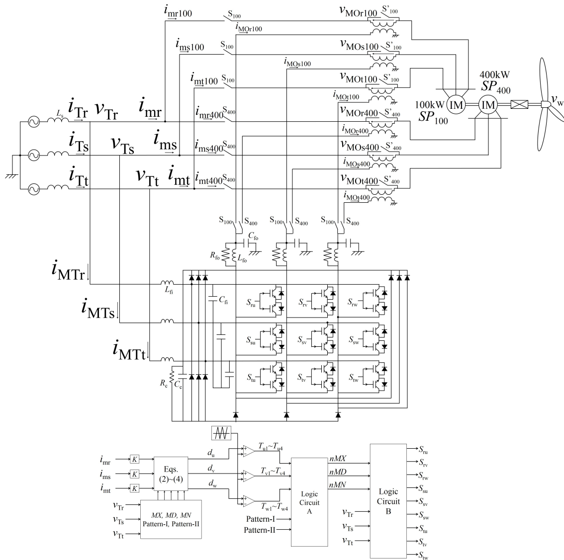
Figure 1. System configuration with the proposed inrush current suppressor using matrix converter (MC) in a large-capacity wind power generation system (WPGS).
