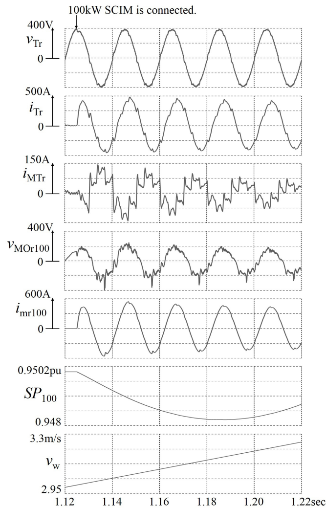
Figure 14. Simulation waveforms with the proposed inrush current suppressor for the 100-kW SCIM.
