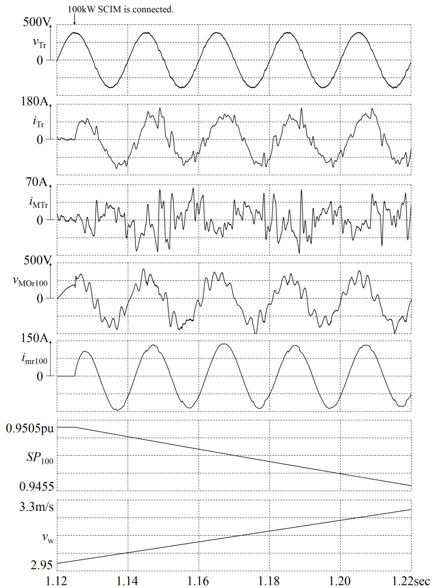
Figure 17. Simulation results with the proposed inrush current suppressor for the 100-kW SCIM when turn ratio is 1:4.
