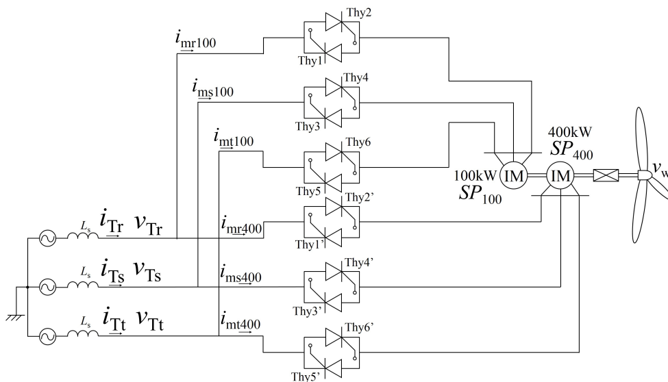
Figure 6. System configuration with the soft-starter in a large-capacity WPGS.
