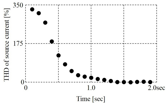
Figure 10. Source current THD of the soft-starter for the 400-kW SCIM in Figure 9.
