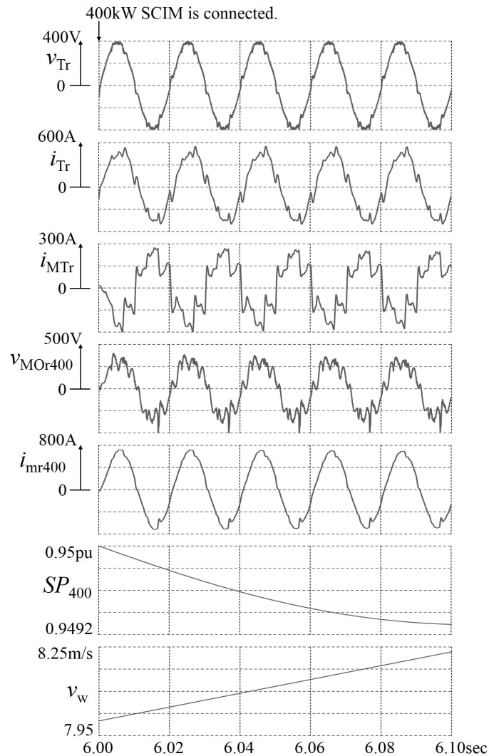
Figure 15. Simulation waveforms with the proposed inrush current suppressor for the 400-kW SCIM.
