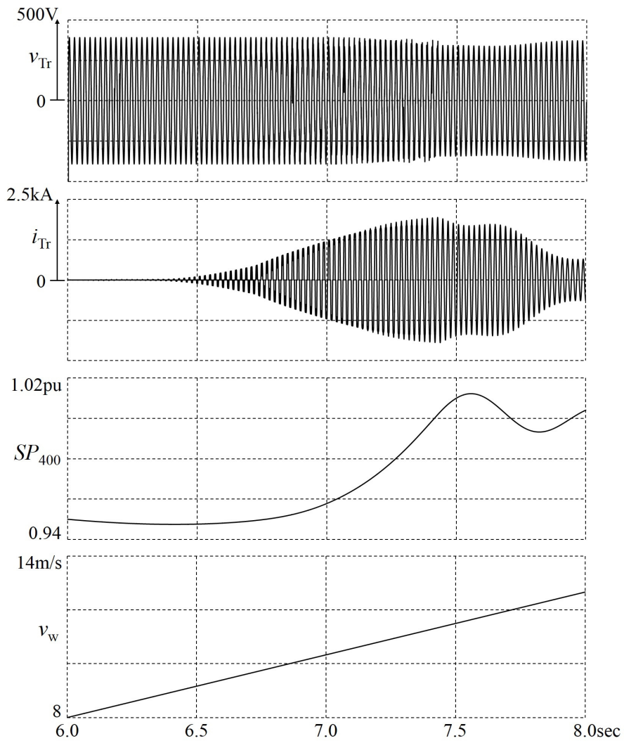
Figure 9. Simulated waveforms with a soft-starter for the 400-kW SCIM.
