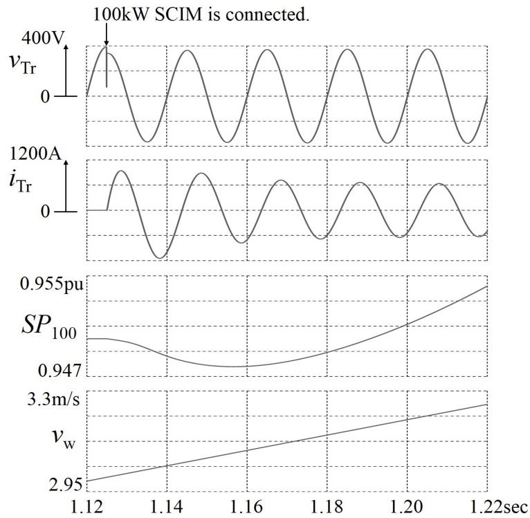
Figure 4. Simulated waveforms of the direct connection for the 100-kW SCIM.
