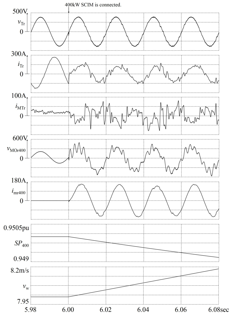
Figure 18. Simulation results with the proposed inrush current suppressor for the 400-kW SCIM when the turn ratio is 1:4.
