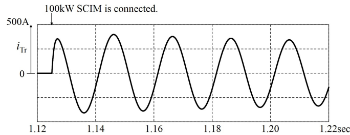
Figure 12. Source current for the 100-kW SCIM with the external resistors.
