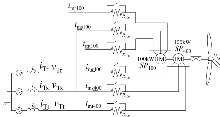
Figure 11. System configuration with external resistors.
