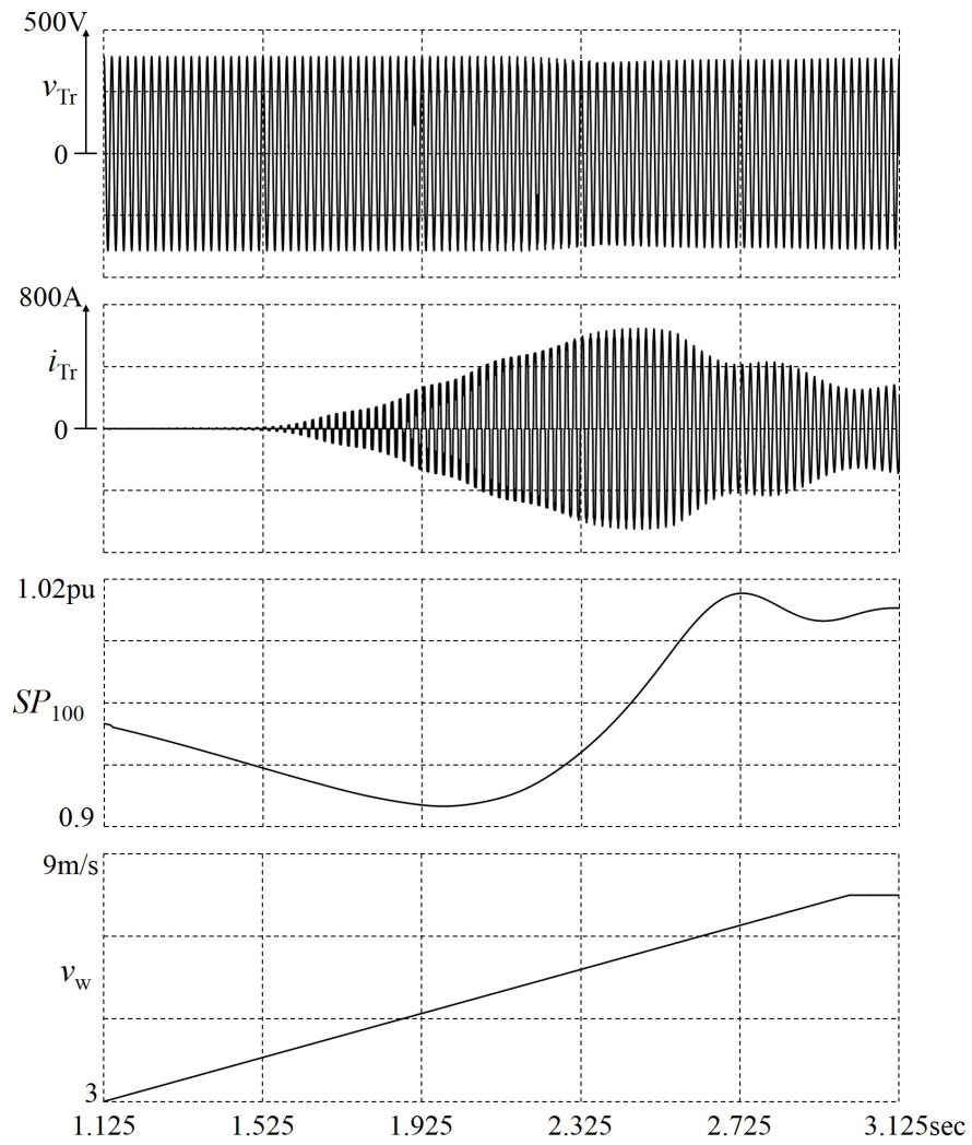
Figure 7. Simulated waveforms with a soft-starter for the 100-kW SCIM.
