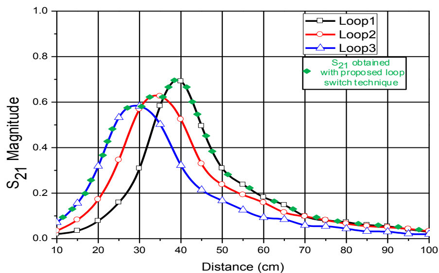
Figure 10. Measured S_{21} magnitude using a vector network analyzer (VNA) for different loops with varying d_{23} in the Case 1 system.
