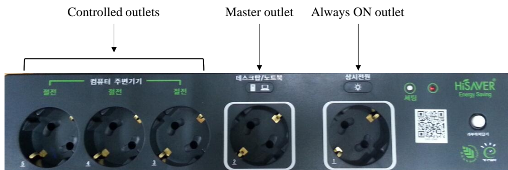
Figure 9. Cutoff device.
