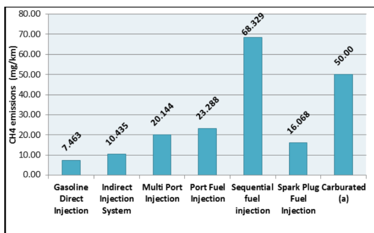
Figure 1. Average CH 4 emissions of different OTTO gasoline fueled of gasoline-blended fueled vehicles equipped with exhaust after treatment system and standard driving conditions. (a No exhaust after treatment system).
