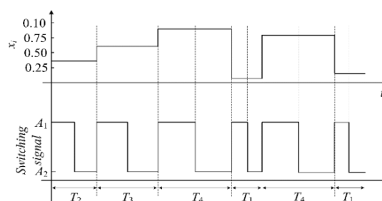
Figure 10. Principle of discretely chaotic modulation.
