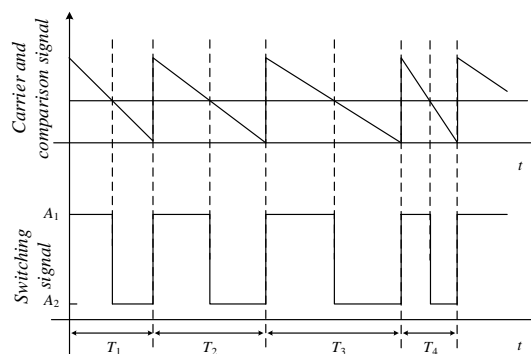
Figure 9. Principle of continuously chaotic modulation.
