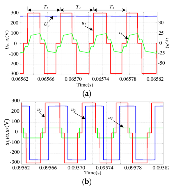
Figure 19. Simulated waveforms of phase-shifted PWM control with continuously chaotic modulation: (a) converter voltage, current of port 1 and output voltage of port 2; (b) converter voltages of port 1, 2 and 3.
