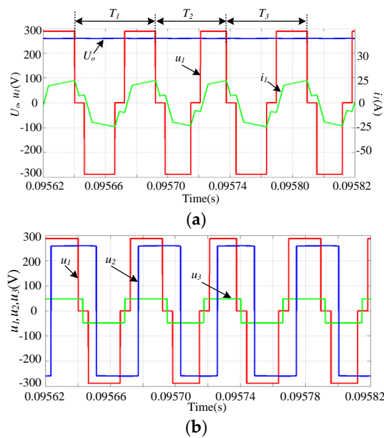
Figure 20. Simulated waveforms of phase-shifted PWM control with discretely chaotic modulation: (a) converter voltage, current of port 1 and output voltage of port 2; (b) converter voltages of port 1, 2 and 3.
