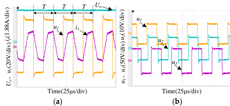
Figure 21. Measured waveforms of shifted-phase angle control using fixed switching-frequency: (a) converter voltage, current of port 1 and output voltage of port 2; (b) converter voltages of port 1, 2 and 3.
