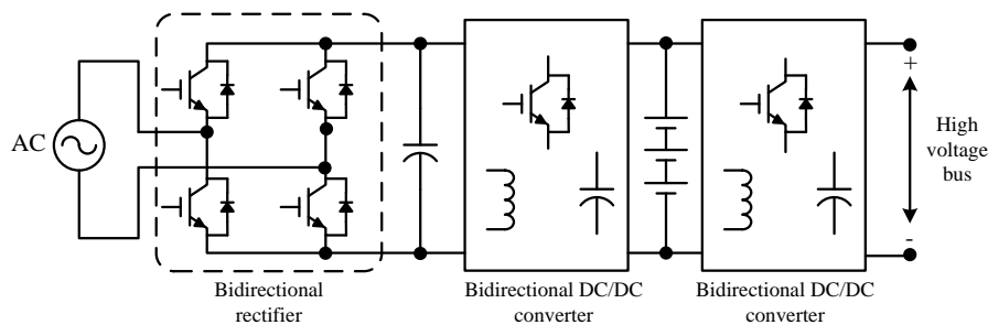
Figure 2. Electric charging system for V2G of EV.
