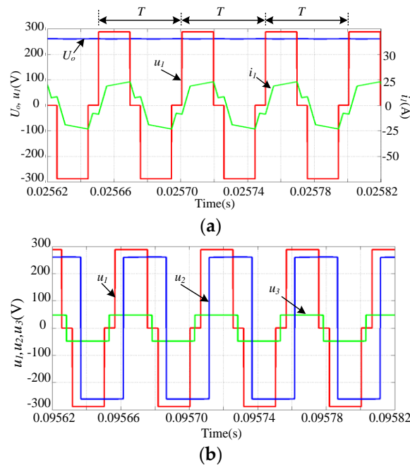
Figure 18. Simulated waveforms of phase-shifted PWM control with fixed switching-frequency: (a) converter voltage, current of port 1 and output voltage of port 2; (b) converter voltages of port 1, 2 and 3.
