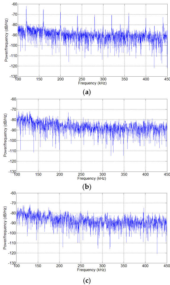
Figure 24. Measured power spectrum density of shifted-phase angle control: (a) fixed switching-frequency; (b) continuously chaotic modulation; (c) discretely chaotic modulation.
