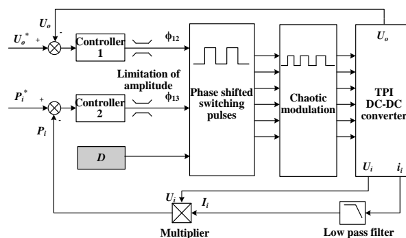
Figure 13. Block diagram of chaotic modulation based control for TPI bidirectional DC/DC converter.
