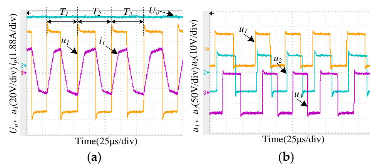
Figure 23. Measured waveforms of shifted-phase angle control using discretely chaotic modulation: (a) converter voltage, current of port 1 and output voltage of port 2; (b) converter voltages of port 1, 2 and 3.
