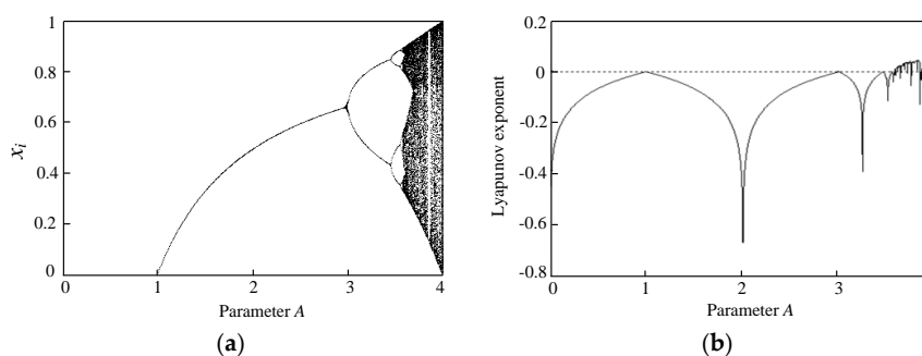
Figure 8. Logistic map: (a) bifurcation diagram; (b) Lyapunov exponents.
