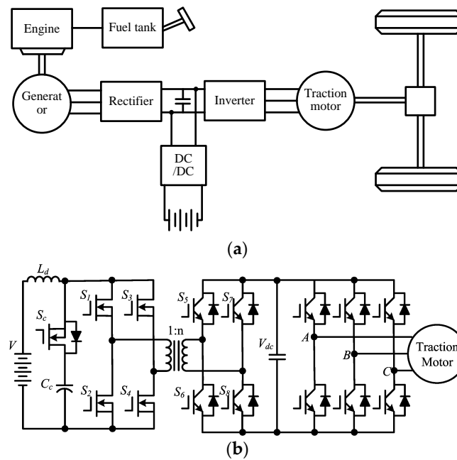
Figure 1. Energy conversion system in series HEV with bidirectional DC/DC converter: (a) system configuration; (b) DAB converter.
