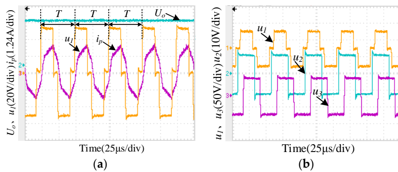
Figure 25. Measured waveforms of phase-shifted PWM control using fixed switching frequency: (a) converter voltage, current of port 1 and output voltage of port 2; (b) converter voltages of port 1, 2 and 3.
