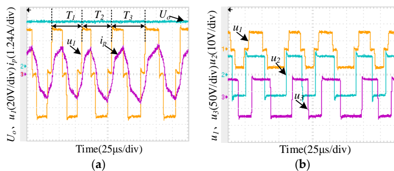
Figure 27. Measured waveforms of phase-shifted PWM control using discretely chaotic modulation: (a) converter voltage, current of port 1 and output voltage of port 2; (b) converter voltages of port 1, 2 and 3.
