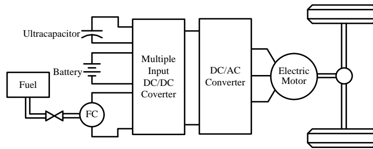
Figure 3. System configuration of fuel cell electric vehicles using multi-input DC/DC converter.
