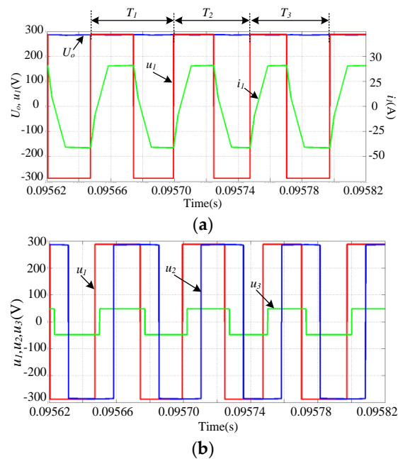
Figure 16. Simulated waveforms of shifted-phase angle control with continuously chaotic modulation: (a) converter voltage, current of port 1 and output voltage of port 2; (b) converter voltages of port 1, 2 and 3.
