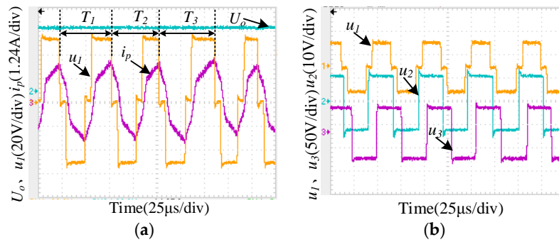
Figure 26. Measured waveforms of phase-shifted PWM control using continuously chaotic modulation: (a) converter voltage, current of port 1 and output voltage of port 2; (b) converter voltages of port 1, 2 and 3.
