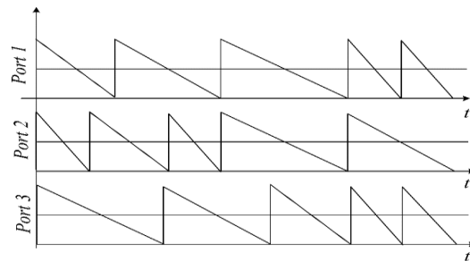
Figure 11. Independently chaotic modulation.
