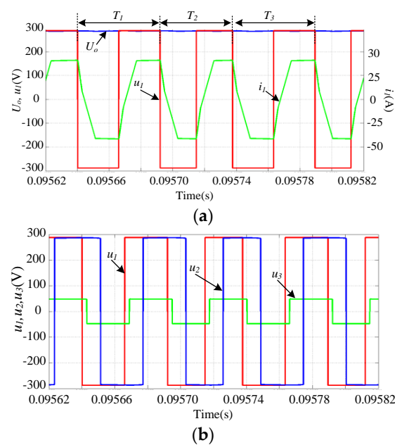
Figure 17. Simulated waveforms of shifted-phase angle control with discretely chaotic modulation: (a) converter voltage, current of port 1 and output voltage of port 2; (b) converter voltages of port 1, 2 and 3.
