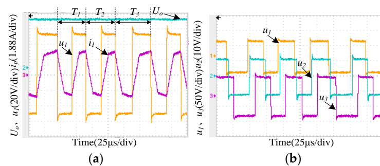
Figure 22. Measured waveforms of shifted-phase angle control using continuously chaotic modulation: (a) converter voltage, current of port 1 and output voltage of port 2; (b) converter voltages of port 1, 2 and 3.
