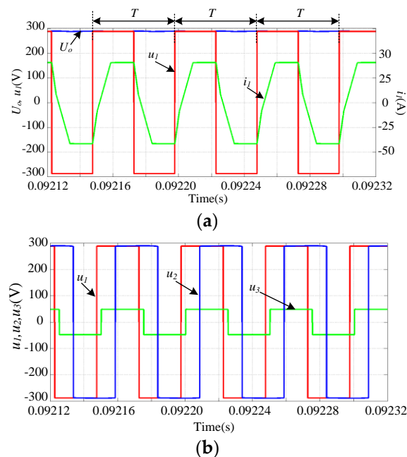
Figure 15. Simulated waveforms of shifted-phase angle control with fixed switching-frequency: (a) converter voltage, current of port 1 and output voltage of port 2; (b) converter voltages of port 1, 2 and 3.
