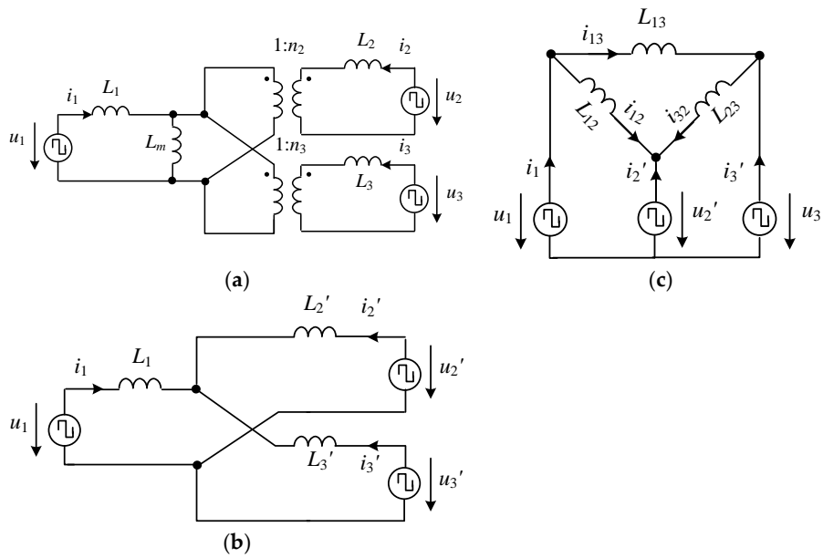
Figure 5. Equivalent model of TPI bidirectional DC/DC converter: (a) original equivalent model with magnetic inductance; (b) simplified Y-type equivalent model observed from port 1 without magnetic inductance; (c) simplified \Delta -type equivalent mode.
