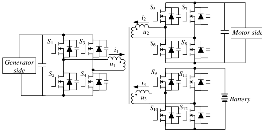
Figure 4. Configuration of TPI bidirectional DC-DC converter.
