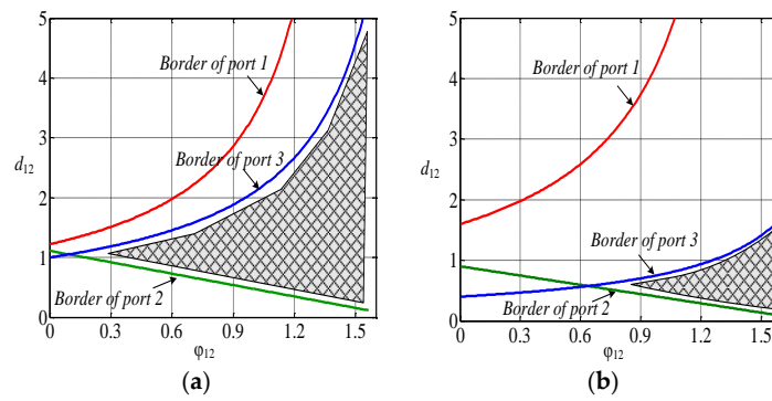
Figure 7. Soft-switching regions for TPI bidirectional DC/DC converter. (a) \phi_{13} = \pi/9, d_{13} = 1 ; (b) \phi_{13} = \pi/6, d_{13} = 0.6 .
