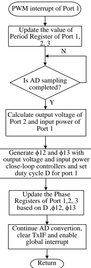
Figure 14. Flow chart of digital implementation for chaotic modulation based control for TPI bidirectional DC/DC converter.
