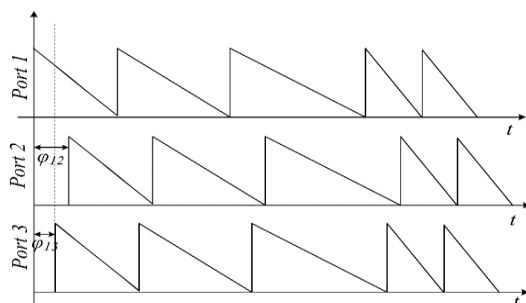
Figure 12. Synchronously chaotic modulation.
