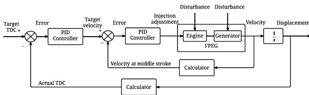
Figure 23. Block diagram FPLG coupled with cascade control [51].
