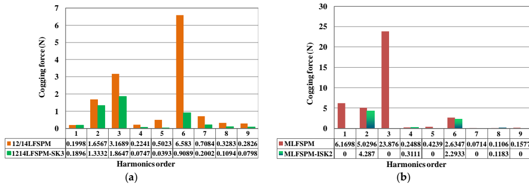
Figure 6. The harmonic distribution comparison of cogging force for: (a) 12/14 LFSM machines; (b) MLFSPM machines.
