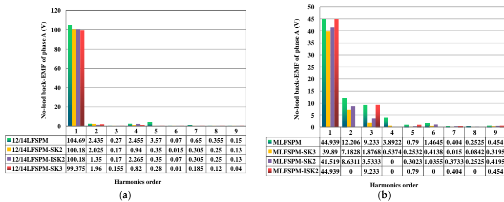
Figure 7. The harmonic distribution of the no-load back-EMFs for: (a) 12/14 LFSM machines; (b) MLFSPM machines.
