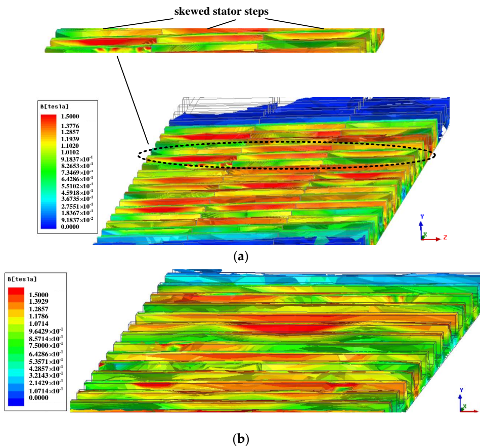
Figure 10. Open-circuit flux density of the stator under 3D FEA for: (a) the 12/14 LFSPM-SK3 machine; (b) 12/14 LFSPM machine.
