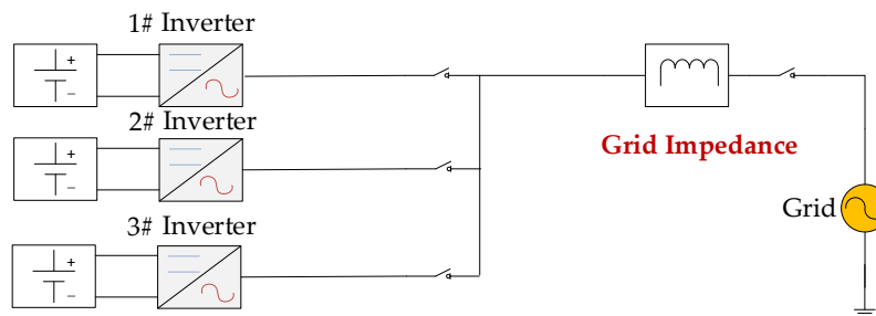
Figure 16. The multi-inverter system with three parallel grid-connected inverters in a weak grid.
