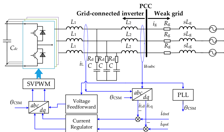
Figure 1. Typical structure of the three-phase grid-connected inverter operating at current source mode (CSM). PLL: phase-locked loop; PCC: point of common coupling; SVPWM: space vector pulse width modulation.
