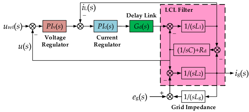
Figure 9. Control block diagram of an inverter operating in VSM.
