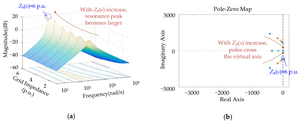
Figure 7. Grid impedance changes in the multi-inverter system with CSM-only control: (a) Bode diagram of G_{\text{CSM}_E}(s) with the grid impedance Z_g(s) changes from 1 p.u. to 6 p.u.; (b) pole-zero map of G_{\text{CSM}_E}(s) with the grid impedance Z_g(s) changes from 1 p.u. to 6 p.u.
