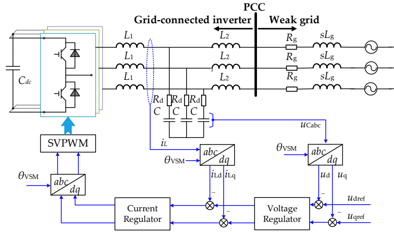
Figure 8. Typical structure of the three-phase grid-connected inverter operating in voltage source mode (VSM).
