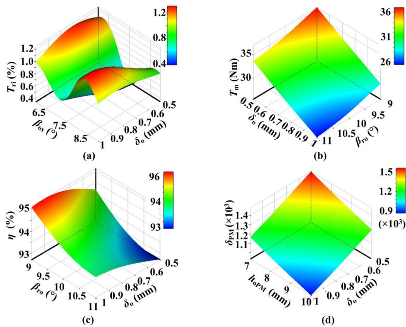
Figure 8. Response of four optimal objects with different key parameters: (a) Response of T_{ri} with \beta_{os} and \delta_o ; (b) Response of T_m in \delta_o and \beta_{ro} ; (c) Response of \eta in \delta_o and \beta_{ro} ; (d) Response of \delta_{PM} in \delta_o and h_{oPM} .
