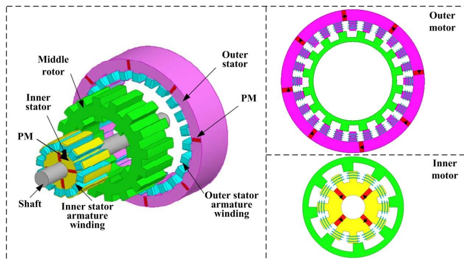
Figure 1. Structure of the DS-PMDS motor.
