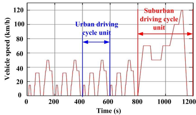
Figure 3. Various driving modes of the DS-PMDS motor in EV.
