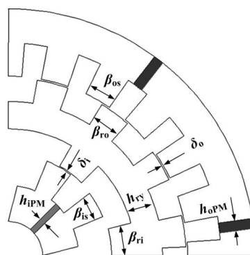
Figure 6. Dimensional parameter model.
