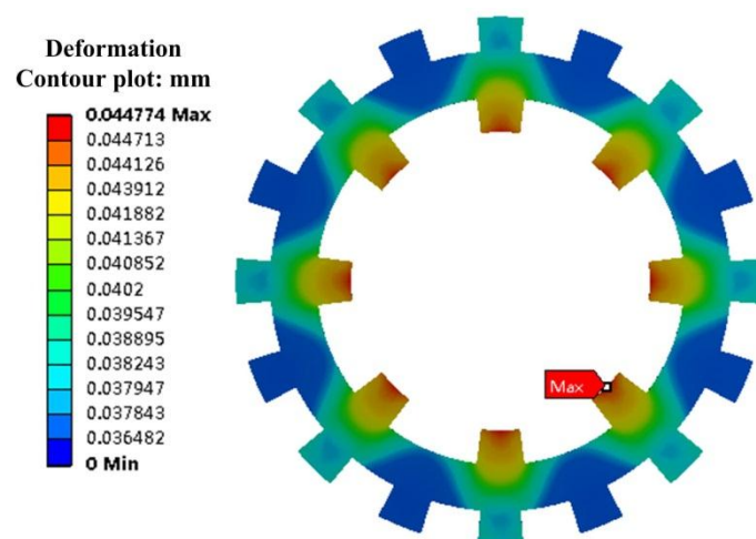
Figure 20. Simulation results for deformation of DS-PMDS motor.
