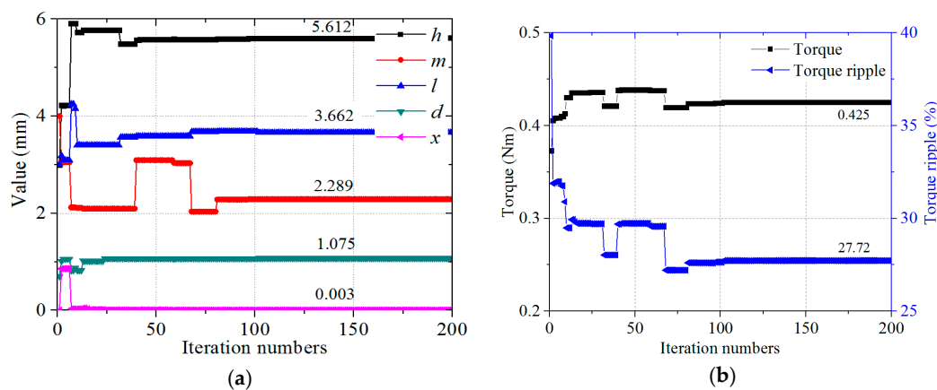
Figure 11. Convergence process: (a) design variables; (b) objective function.
